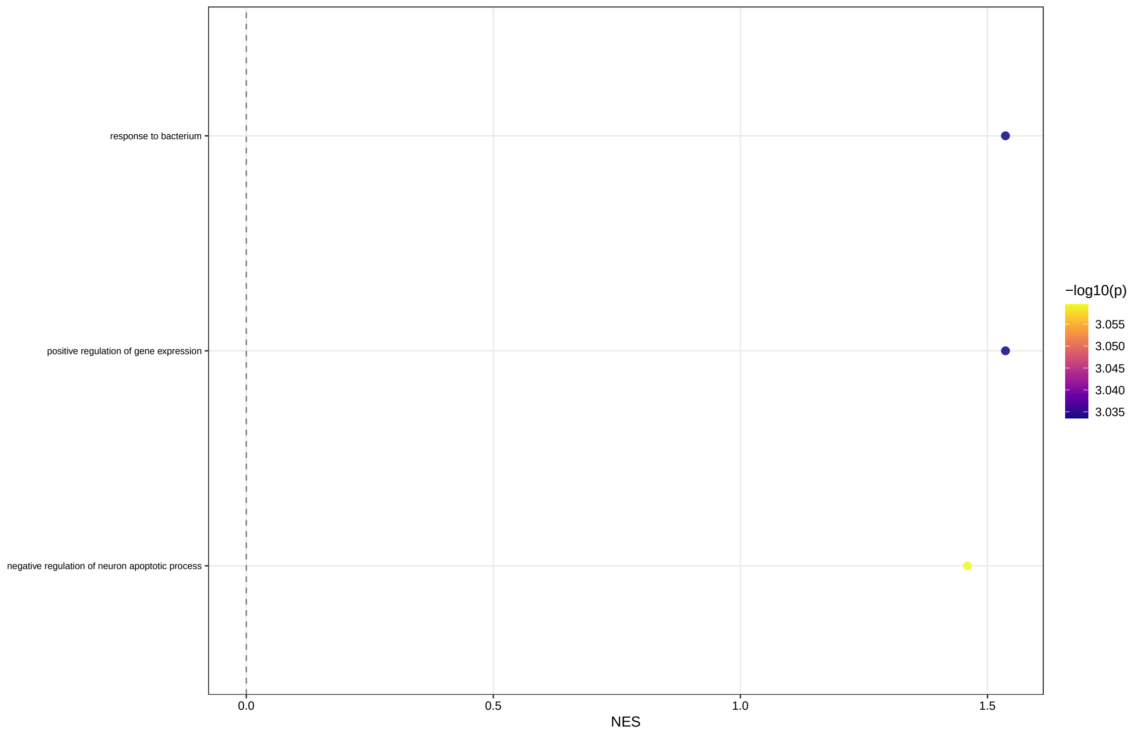
GO:BP GSEA – Nuclear factor 1 (3 terms)
