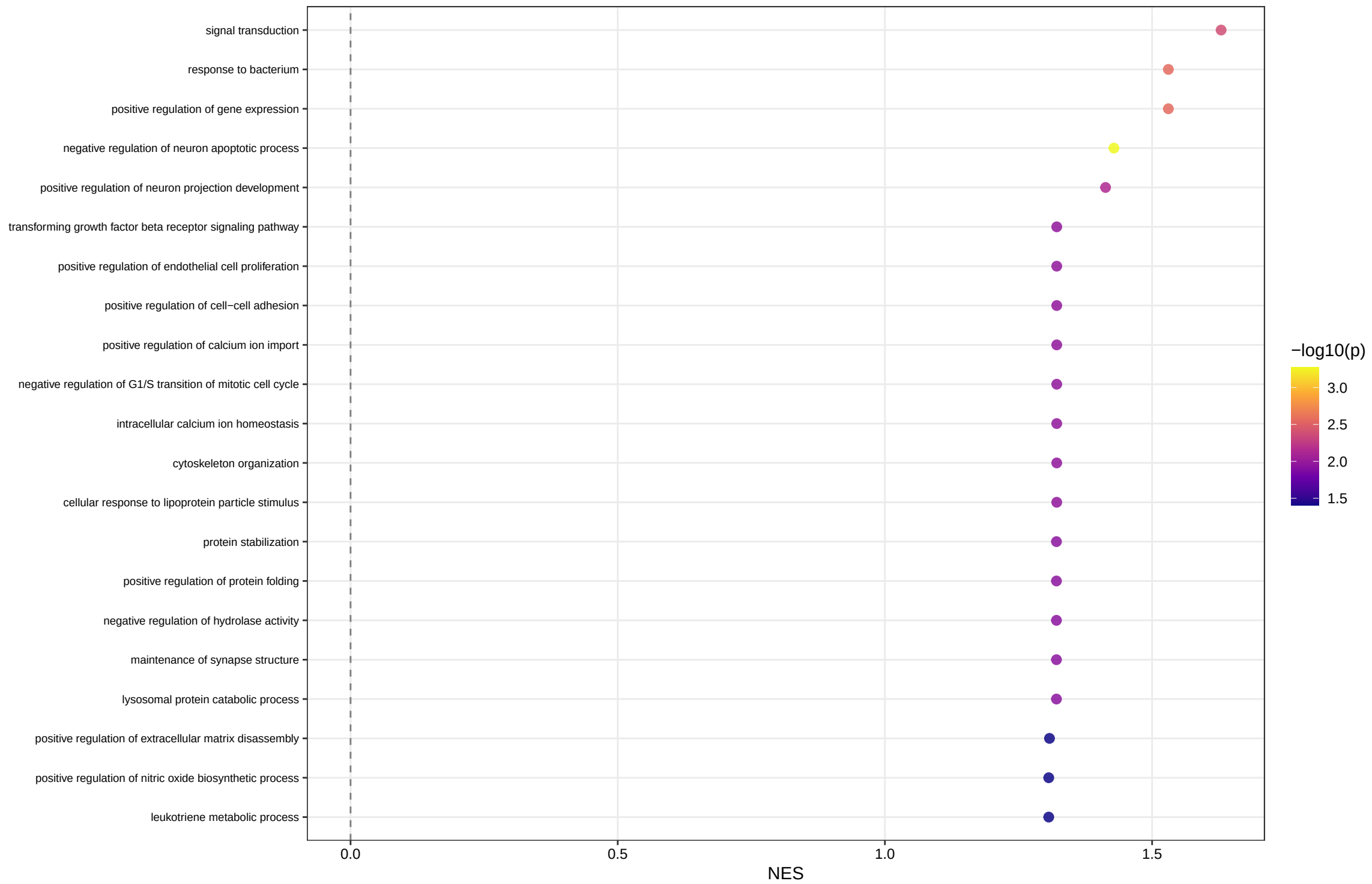
GO:BP fgsea – Nuclear factor 1 (21 terms)
