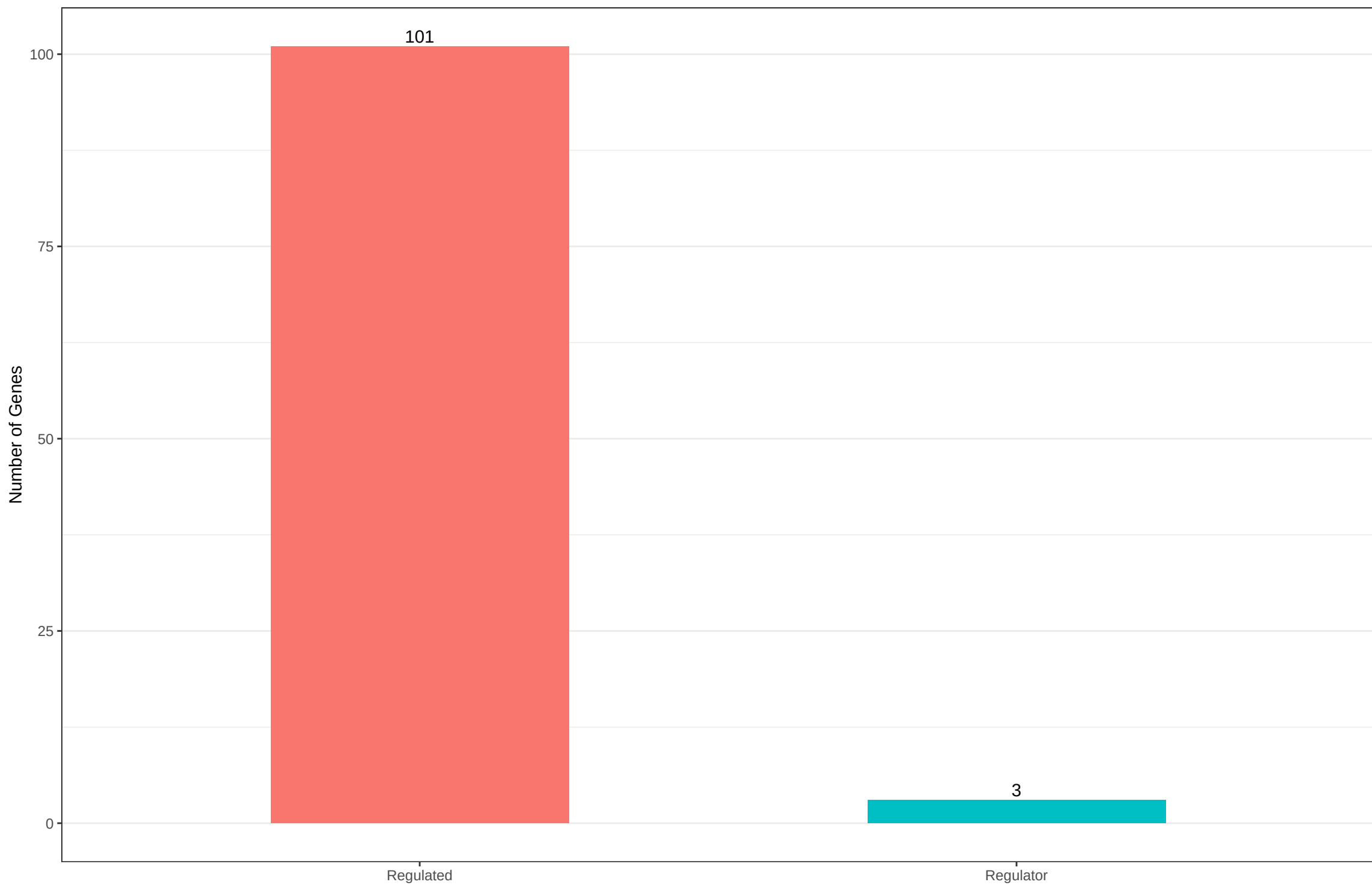
Network Composition – Runt-related factors
