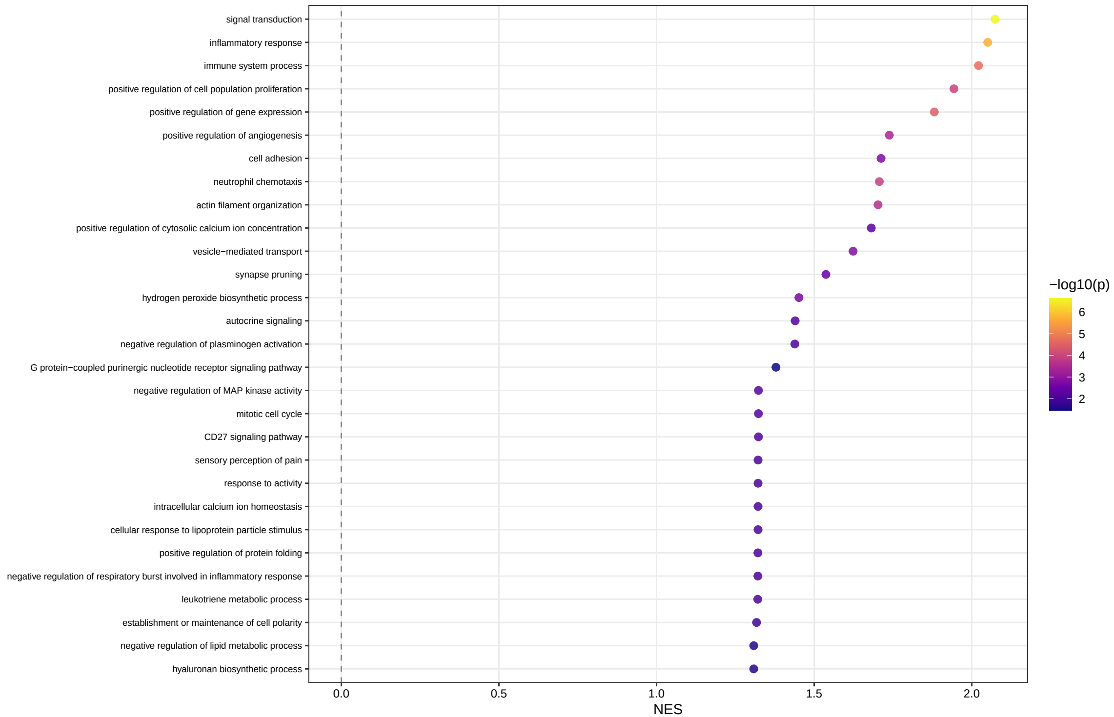
GO:BP fgsea – Runt-related factors (29 terms)
