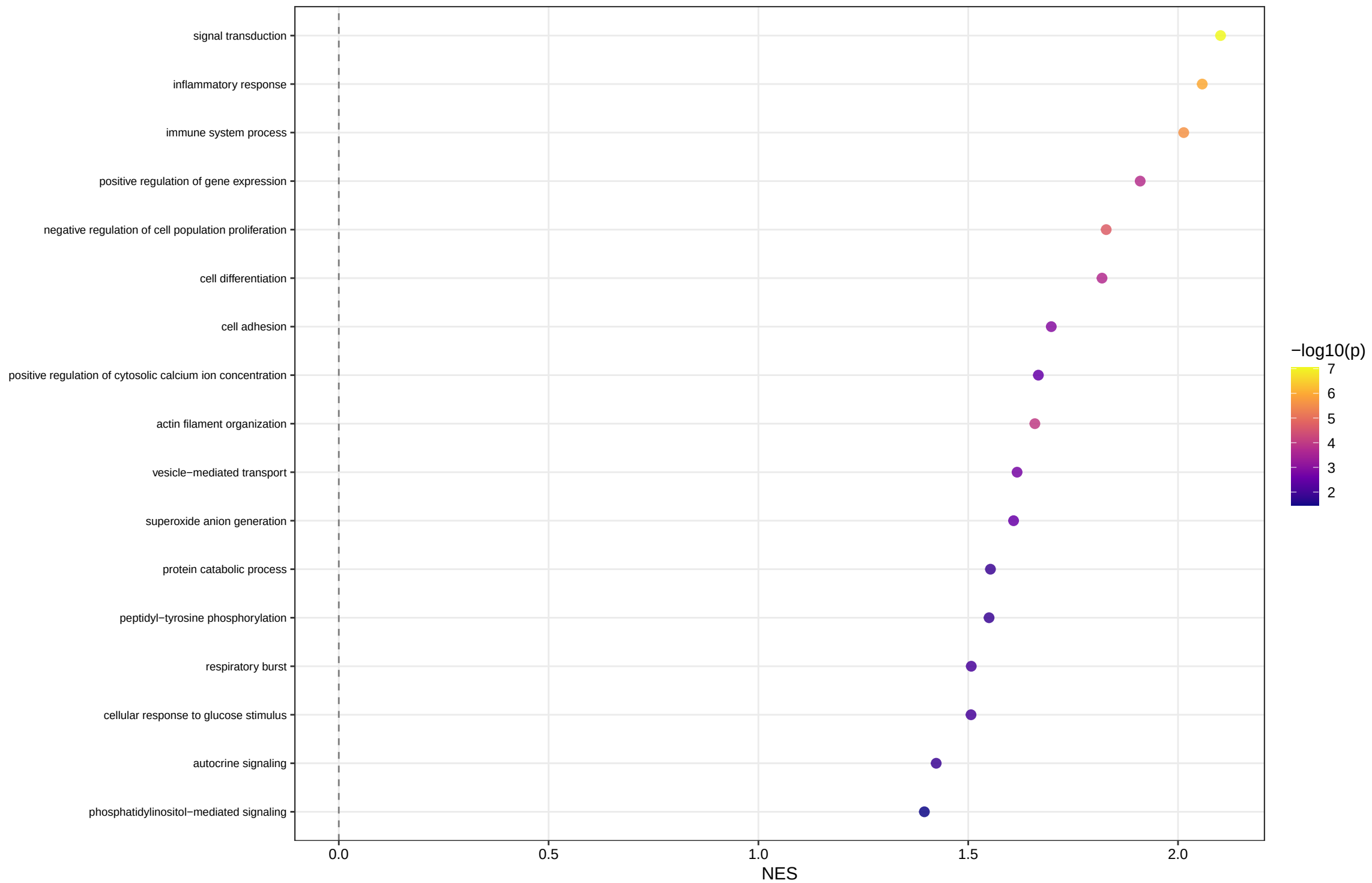
GO:BP GSEA – Runt-related factors (17 terms)
