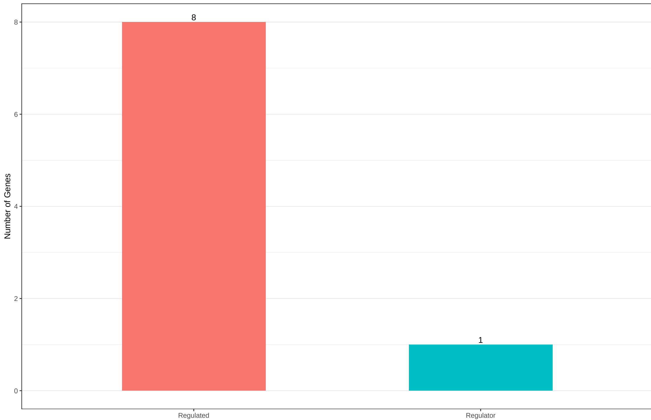
Network Composition – SOX-related factors
