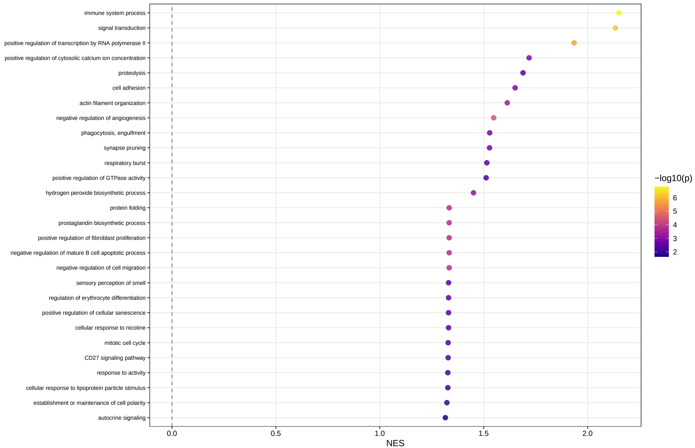
GO:BP fgsea – TBP-related factors (28 terms)
