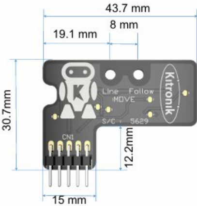
Figure 1: Kitronik 5629 Line Follower Board
