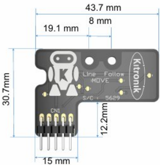
The Line follower board is 5.7mm front to back
