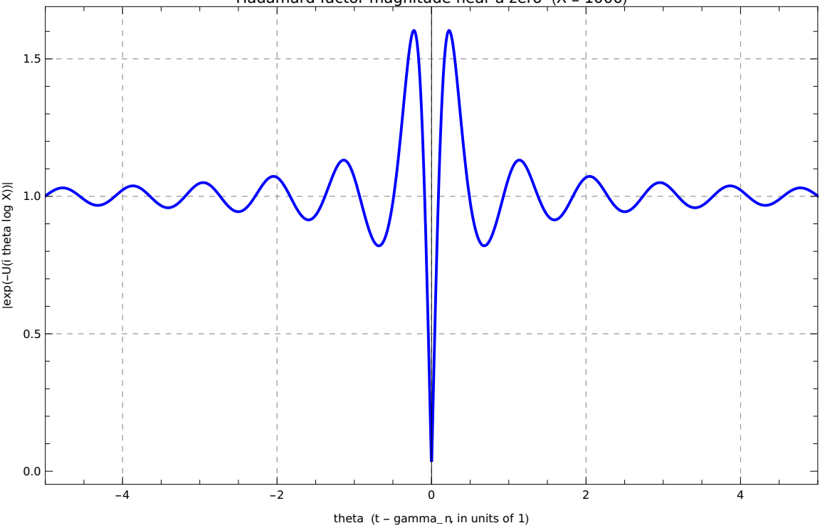
Hadamard factor magnitude near a zero (X = 1000)
