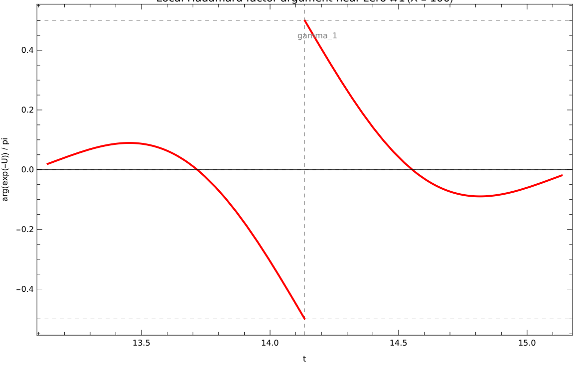
Local Hadamard factor argument near zero #1 (X = 100)
