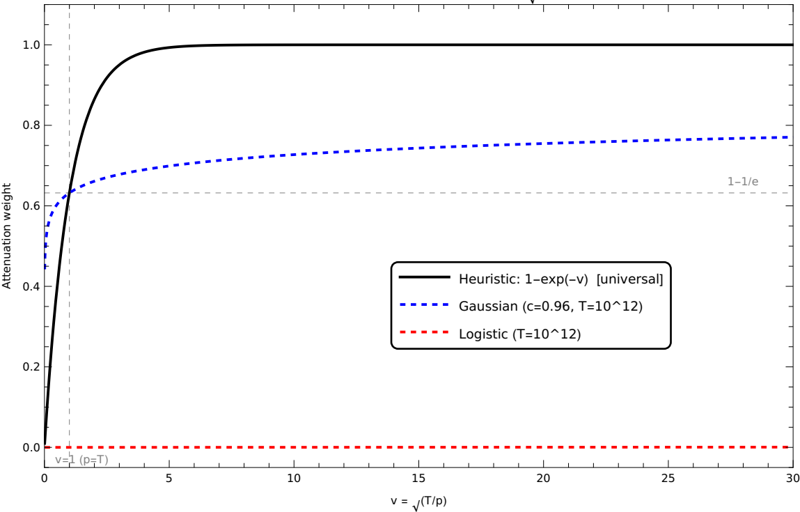
Attenuation in natural variable v = \sqrt{T/p}
