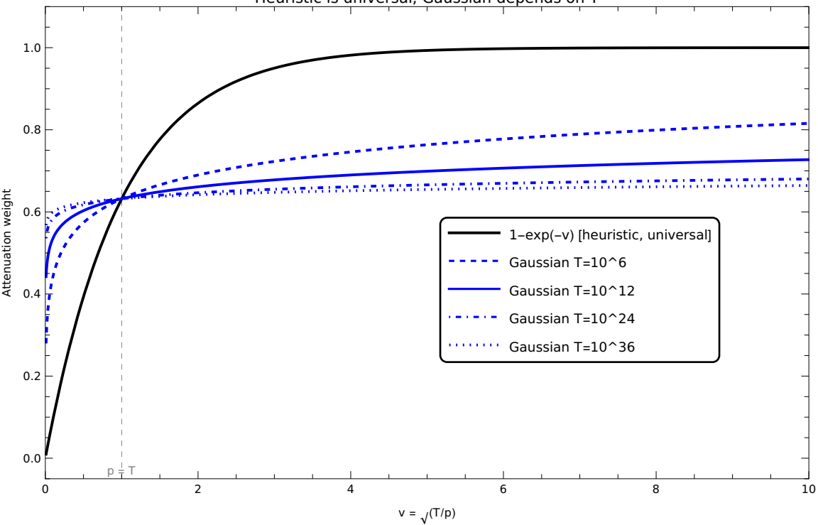
Heuristic is universal; Gaussian depends on T
