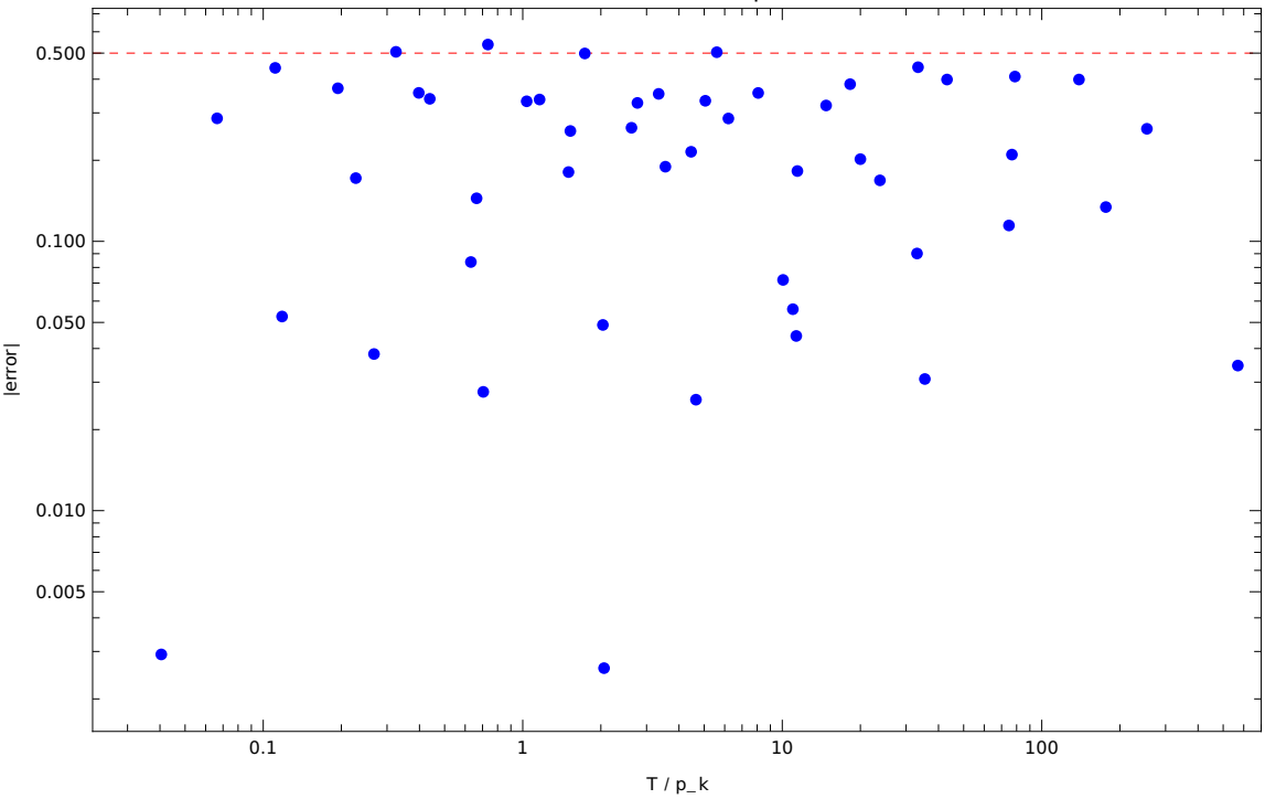
Truncation error vs T/p_k ratio
