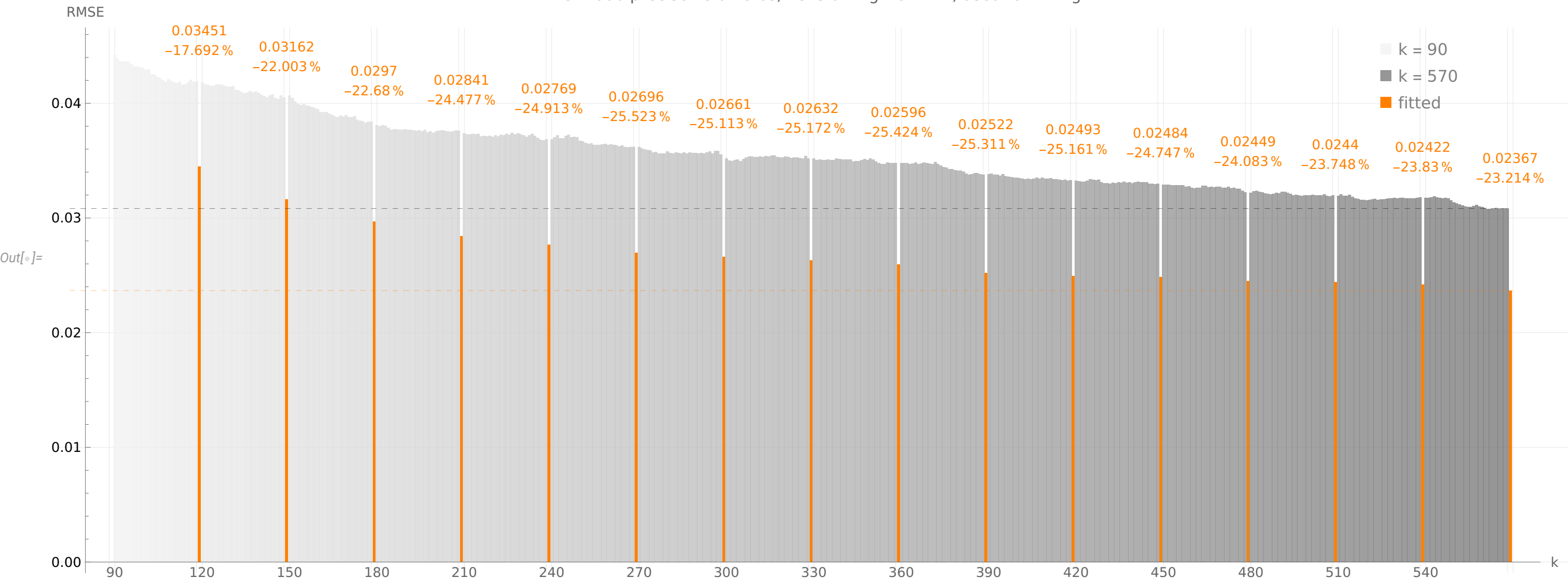
RMSE of 1000 zzz approximated zeros after \#10^5 First 1000 precise zeta zeros, i.e. starting from \#1 , used for fitting
