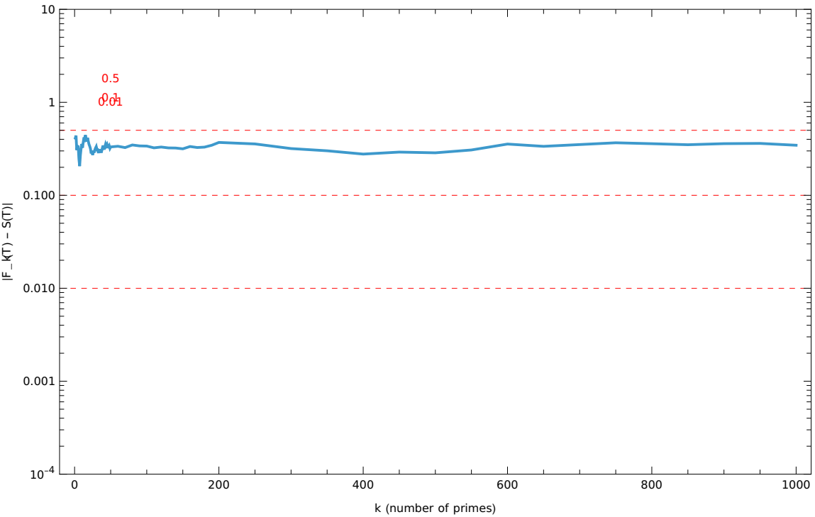
Truncation error at T ~ 237
