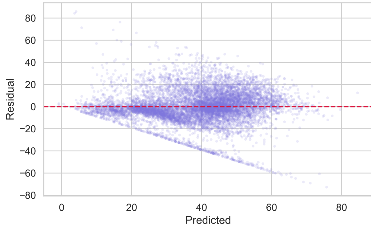
LightGBM: Residuals
