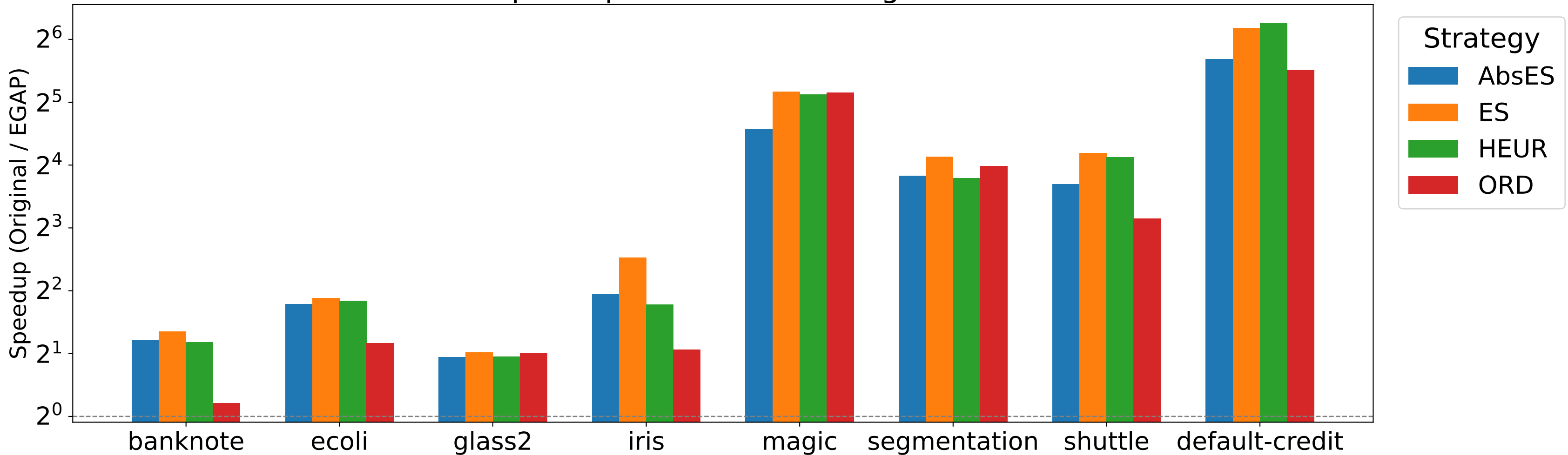
Speedup of EGAP over Original
