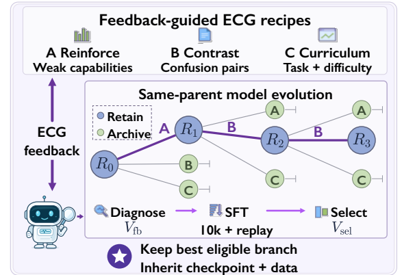
Figure 3 Schematic of feedback-guided model evolution. A/B/C change category coverage, confusion contrasts, or difficulty/task mixtures. Each candidate adds 10,000 accepted questions plus replay. Purple shows an illustrative lineage. Table 13 reports measured mixtures, scores, and choices.
