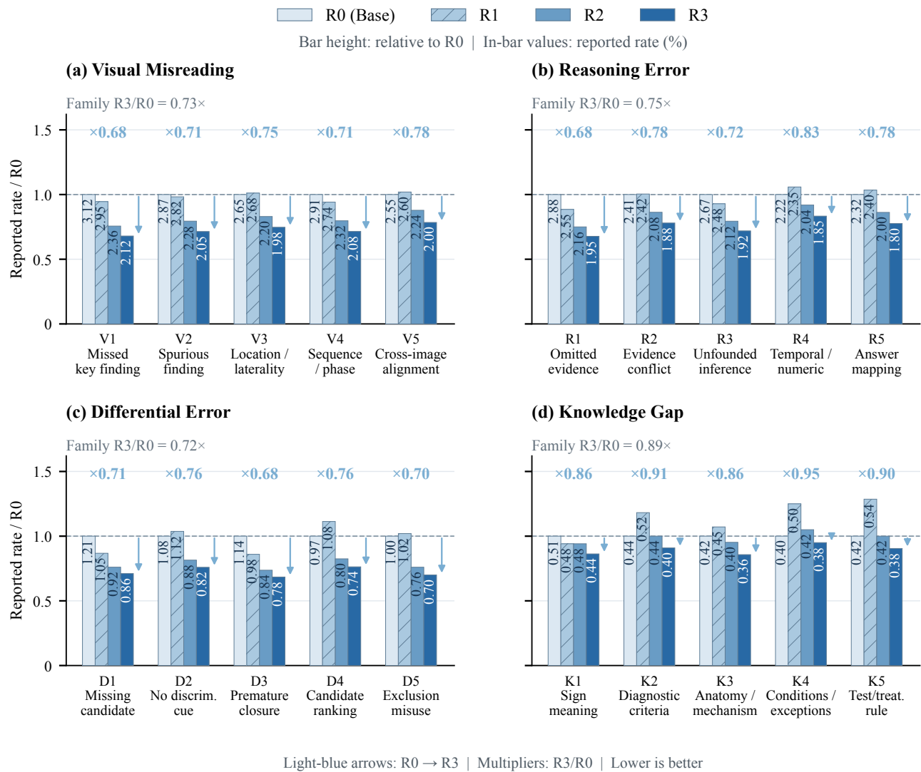
Figure 7 Twenty error subtypes of the 9B model across R0–R3. Each panel contains five subtypes. Bar heights divide reported rates by the corresponding subtype’s R0 rate; in-bar labels give original percentages. Light-blue arrows and multipliers show R3 relative to R0, with lower values indicating larger relative reductions. Family R3/R0 is the ratio of the summed subtype rates. Horizontal codes such as R1–R5 denote reasoning-error subtypes, distinct from round labels R0–R3 in the legend.
