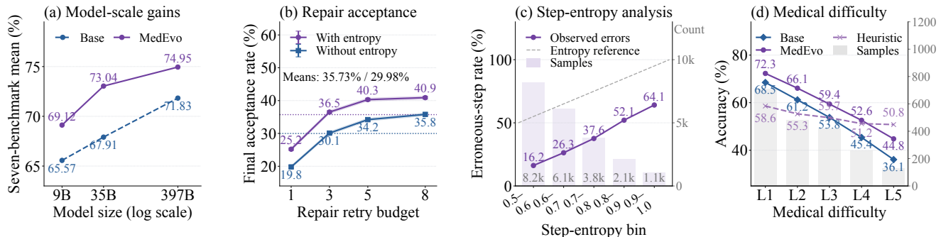
Figure 6 Scale, uncertainty, and difficulty. (a) Mean accuracy after R3 for 9B/35B and R2 for 397B. (b) Repair acceptance with/without entropy localization; pointwise 95% Wilson intervals use 45,000 attempts per setting. (c) Error rates and step counts by entropy bin; the diagonal is a numerical reference. (d) Accuracy by difficulty; sample counts use the right axis.
