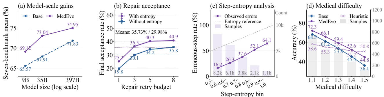
Figure 6 Scale, uncertainty, and difficulty. (a) Mean accuracy after R3 for 9B/35B and R2 for 397B. (b) Repair acceptance with/without entropy localization; pointwise 95% Wilson intervals use 45,000 attempts per setting. (c) Error rates and step counts by entropy bin; the diagonal is a numerical reference. (d) Accuracy by difficulty; sample counts use the right axis.
