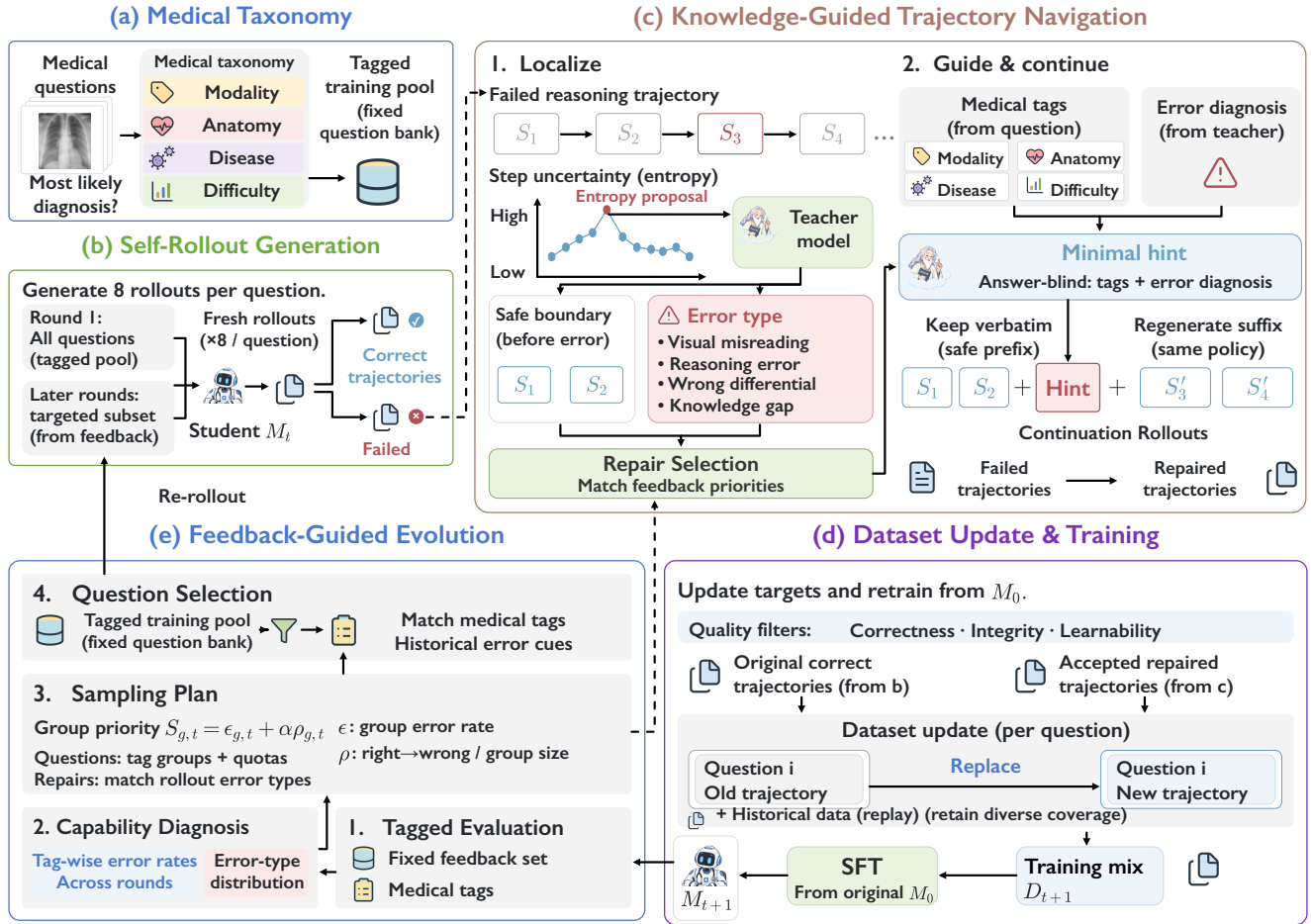
Figure 4 Knowledge Navigation in MedEvo. (a) Medical tags organize questions. (b) The current student generates fresh rollouts. (c) Knowledge-guided trajectory navigation localizes errors and provides recovery hints through a gold-blind auditor; the student preserves the valid prefix and regenerates the suffix. (d) Admitted trajectories update the training set, retaining valid historical targets; the next model trains from M_0 . (e) Fixed-set feedback guides question selection for the next round.
