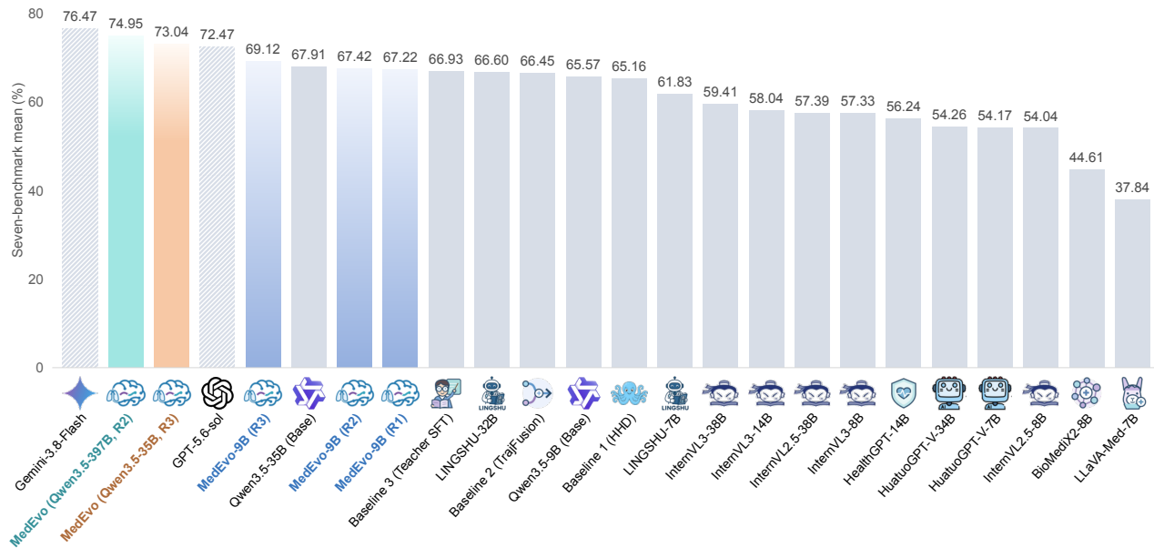
Figure 1 Medical multimodal reasoning across model scales. Mean accuracy on seven benchmarks. MedEvo improves Qwen3.5 models with 9B, 35B, and 397B parameters. B: billion parameters; supervised fine-tuning (SFT); Hindsight Hint Distillation (HHD) [1].
