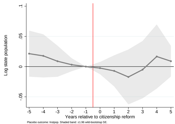
(b) Log State Population
