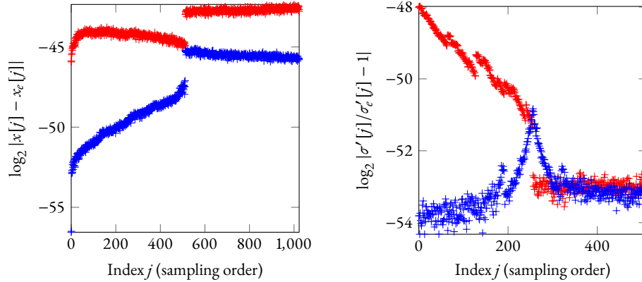
Fig. 1: Average deviations of centres x and widths \sigma' from exact values of the “standard” (red) and new (blue) implementations ( n = 512 ).
