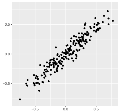
Scatter plot of differences
