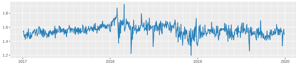
Second residual time series
