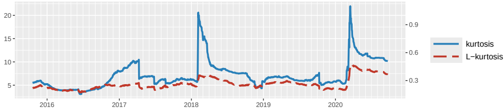
Comparison of (normalized) fourth moments
