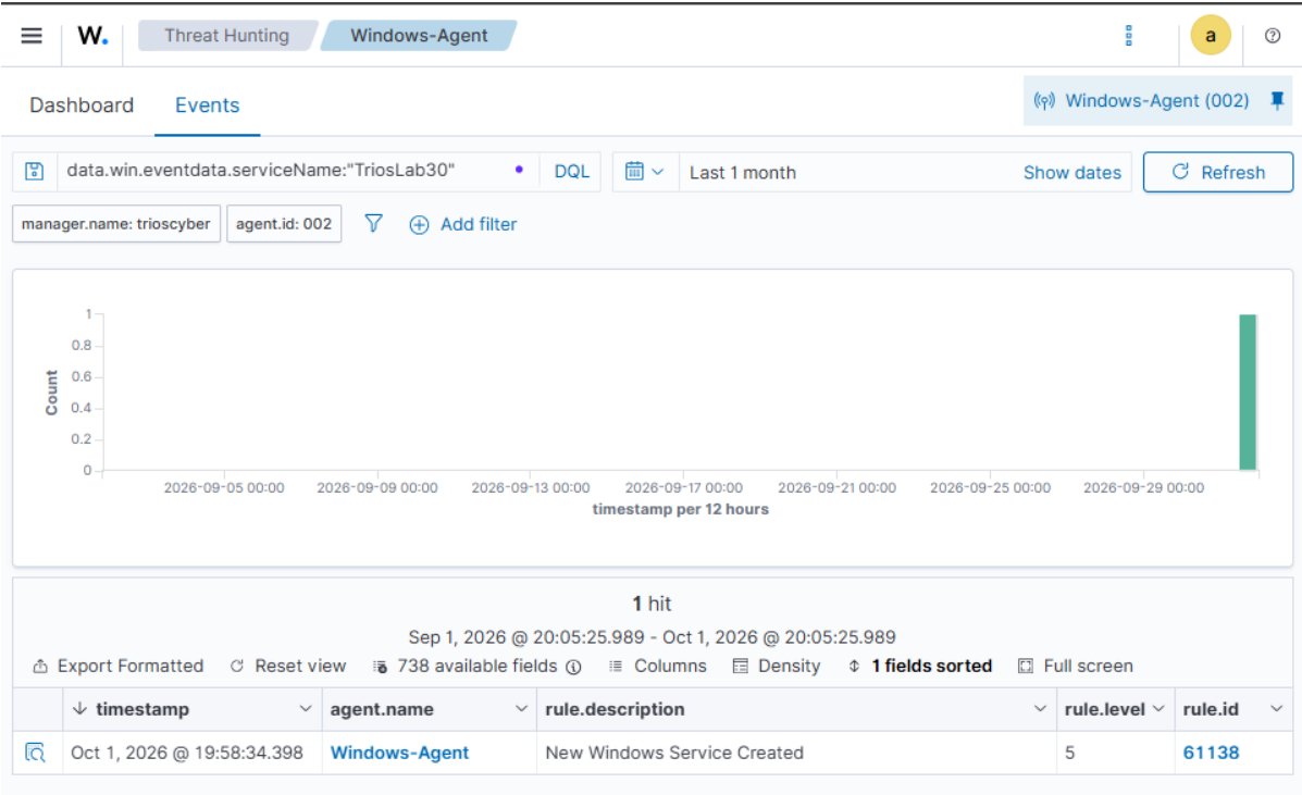
Wazuh alert generated for the TriosLab30 service-creation event.
