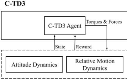
Fig. 6. The C-TD3 agent's block diagram.
