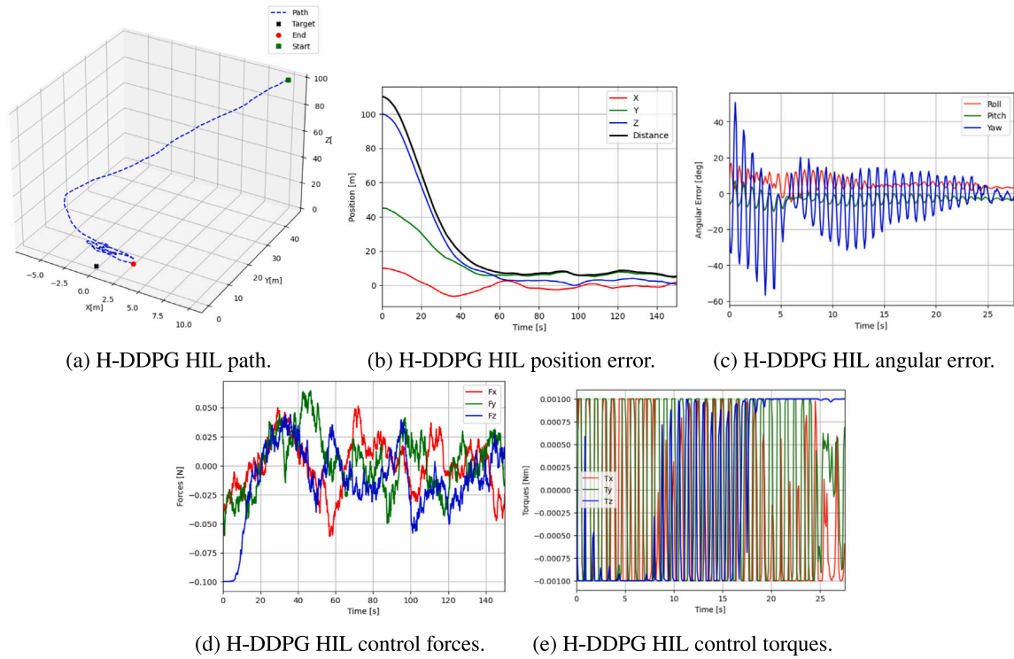
Fig. 19. HIL results for the H-DDPG control system.
