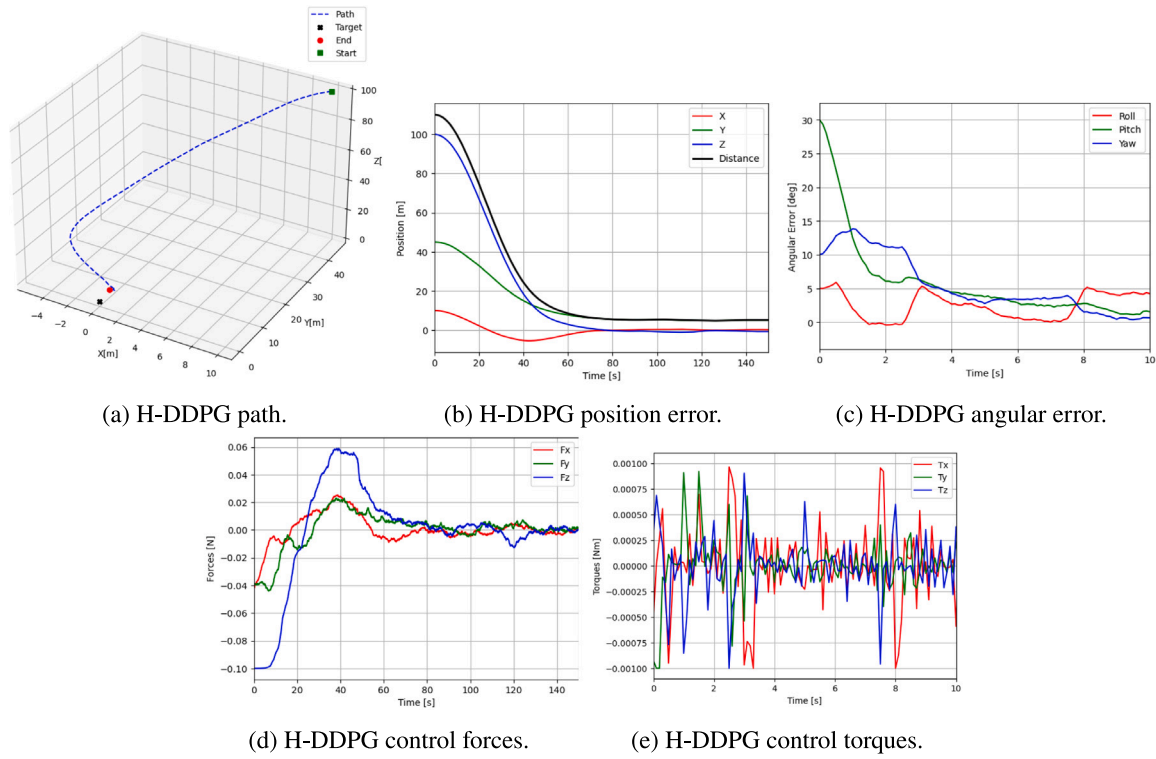
Fig. 10. Simulation results for the H-DDPG control system.
