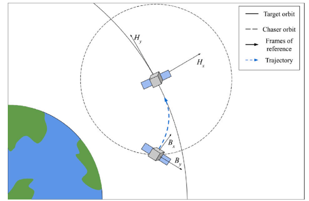
Fig. 1. An illustration of the Hill frame commonly used for the Clohessey–Wiltshire equations.
