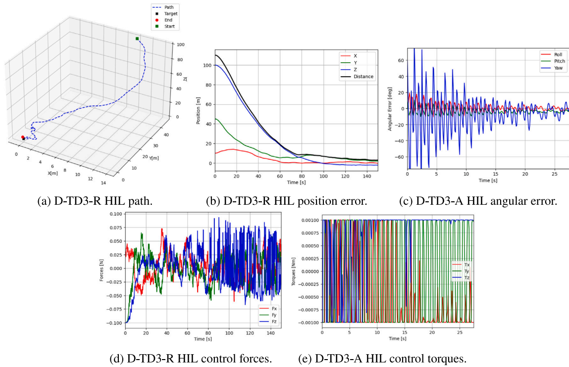
Fig. 18. HIL results for the TD3 control system.
