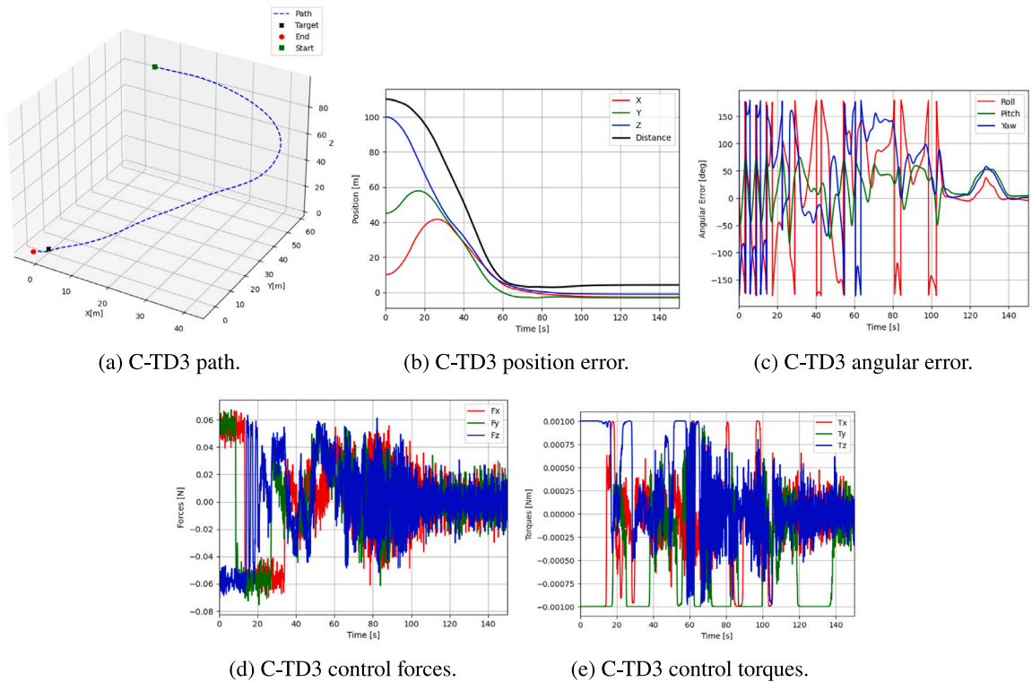
Fig. 9. Simulation results for the C-TD3 control system.
