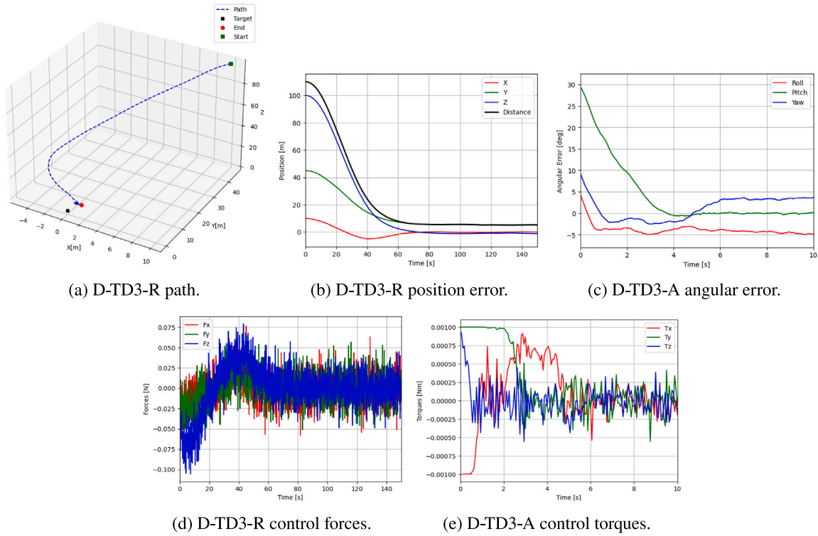
Fig. 8. Simulation results for the D-TD3 control system.
