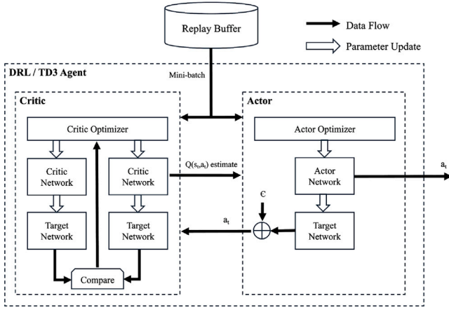
Fig. 4. The structure of a TD3 agent.
