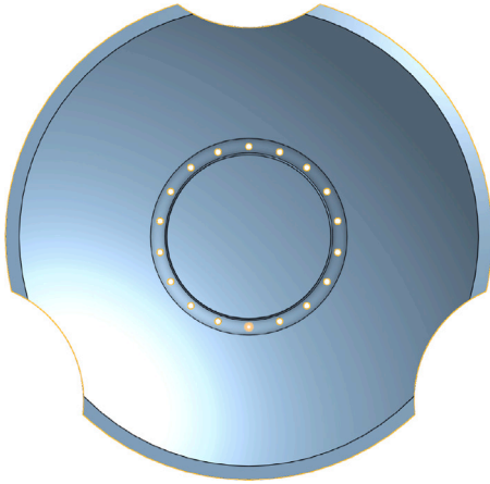
Fig. 15. Top view of the stator.
