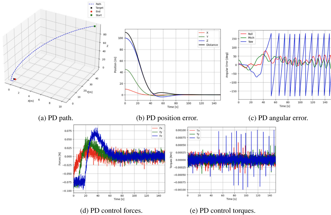
Fig. 11. Simulation results for the classical PD control system.
