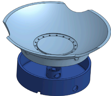
Fig. 14. The two piece stator design.
