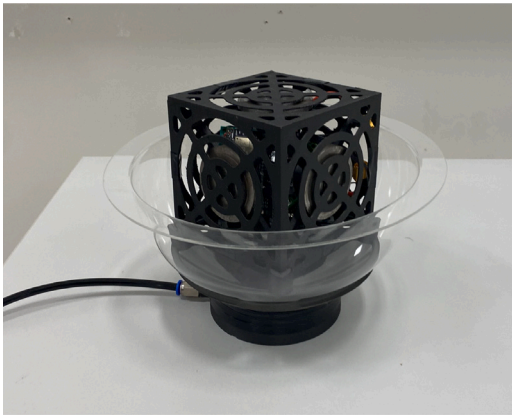
Fig. 16. The completed attitude dynamics testing platform.
