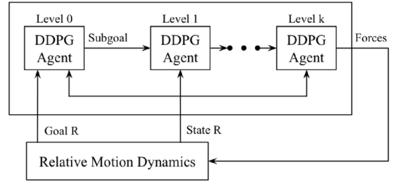
Fig. 7. The H-DDPG agent's block diagrams.
