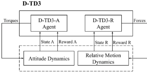
Fig. 5. The D-TD3 agent's block diagram.
