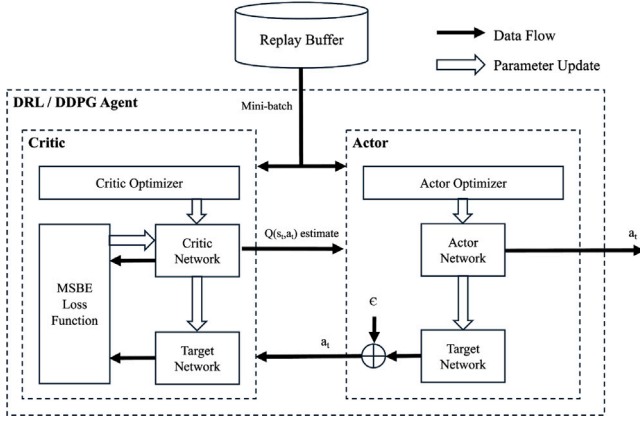
Fig. 3. The structure of a DDPG agent.
