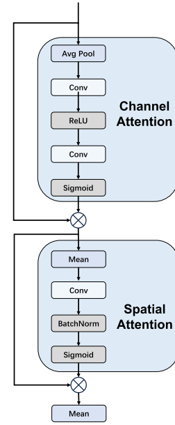
(b) CBAM Attention Module
