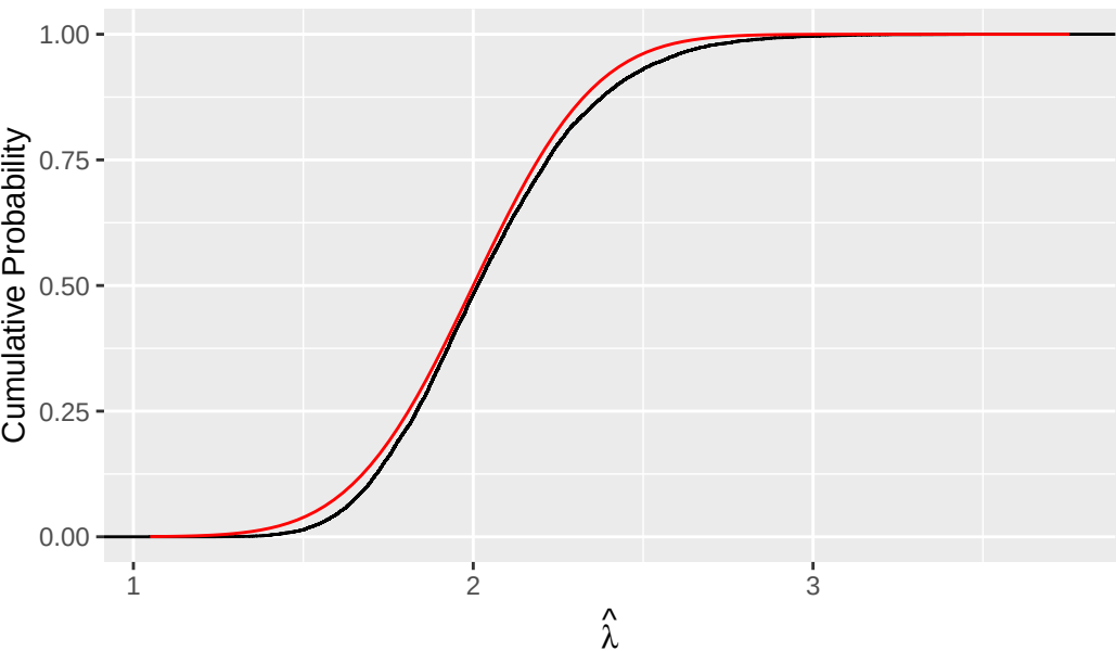
ECDF of Simulated ML Estimates vs Asymptotic Sampling Dis
