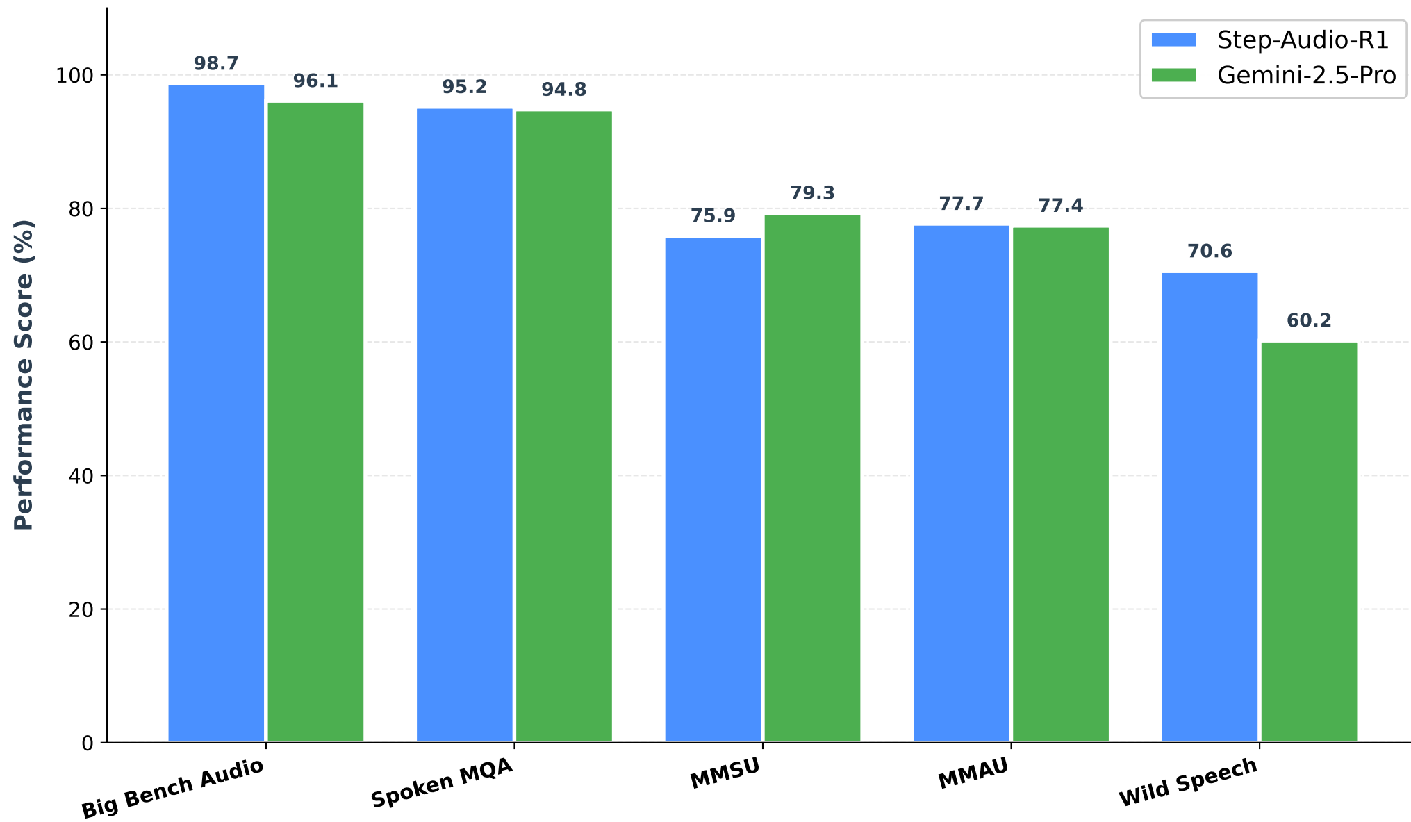
S2T Benchmark
