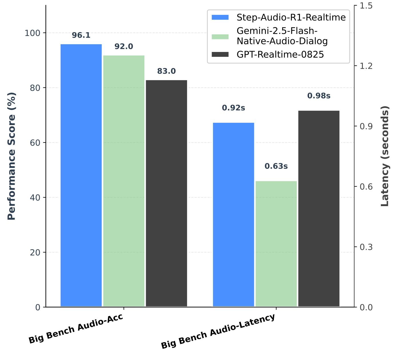
S2S Benchmark
