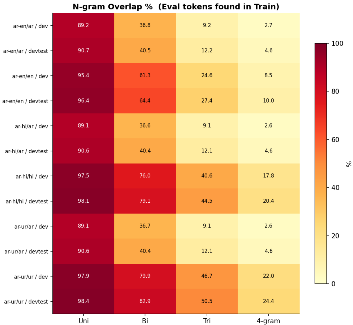
N-Gram Overlap Heatmap (Train vs Eval)
