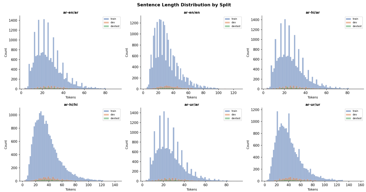
Sentence Length: Train vs Dev vs DevTest
