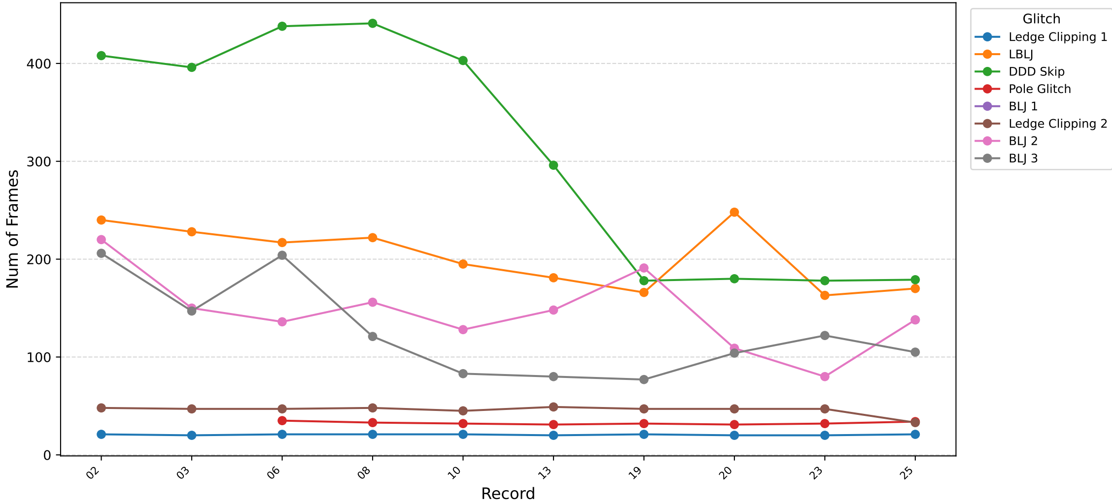
Frame Count Transition of Each Glitch in SM64 0-Star Speedrun Categories
