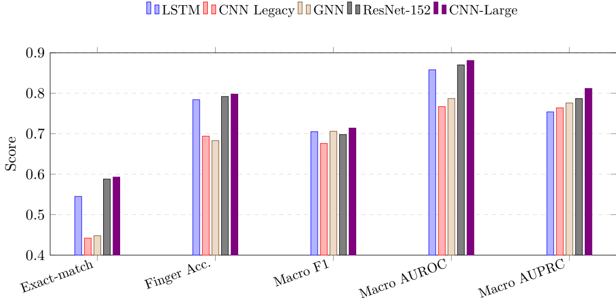
Figure 2: Aggregate-metric comparison across the three direct baselines plus the strongest internal teacher and student references from the newer CNN branch.
