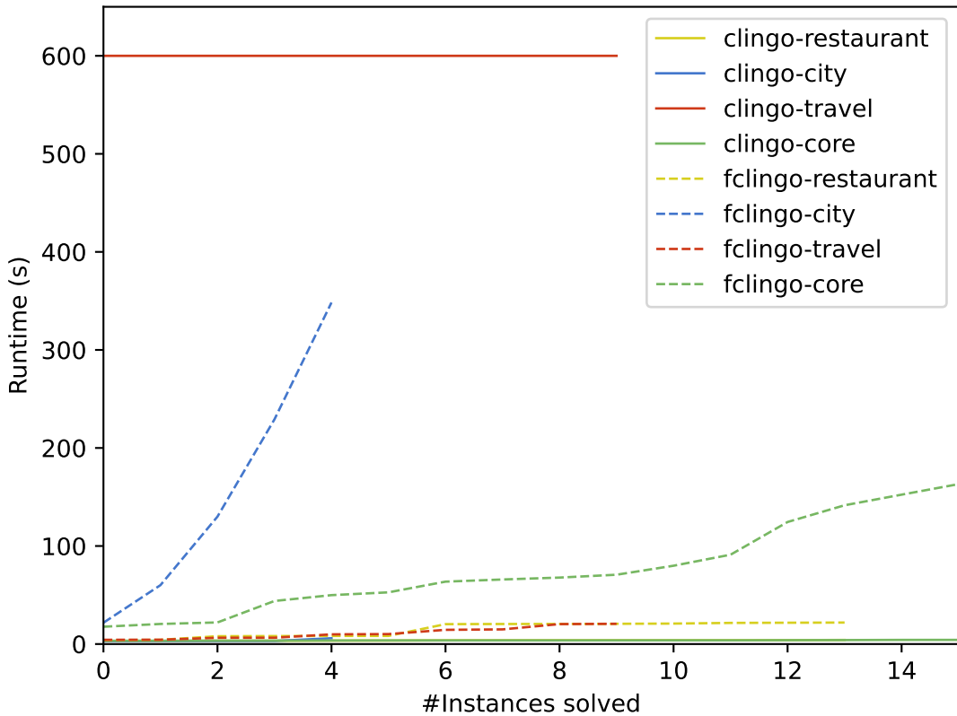
Cactus plot of all benchmarks
