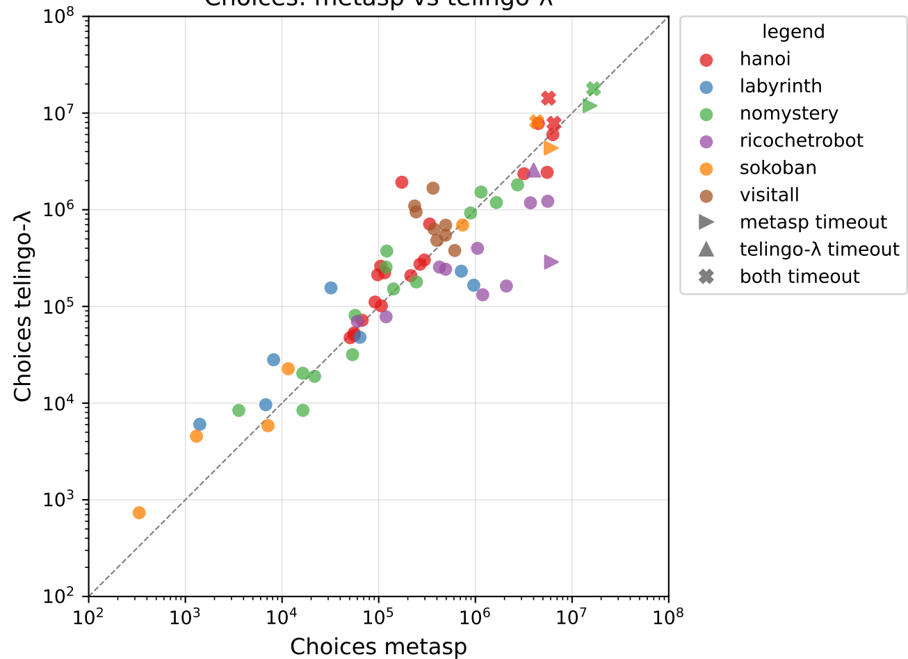
Choices: metasp vs telingo- \lambda
