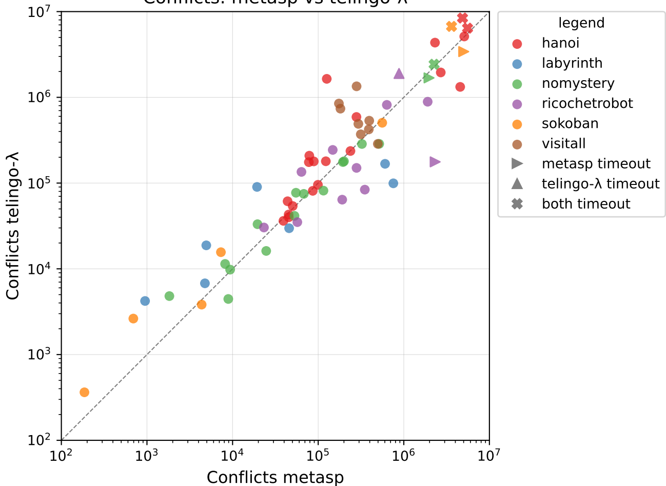
Conflicts: metasp vs telingo- \lambda
