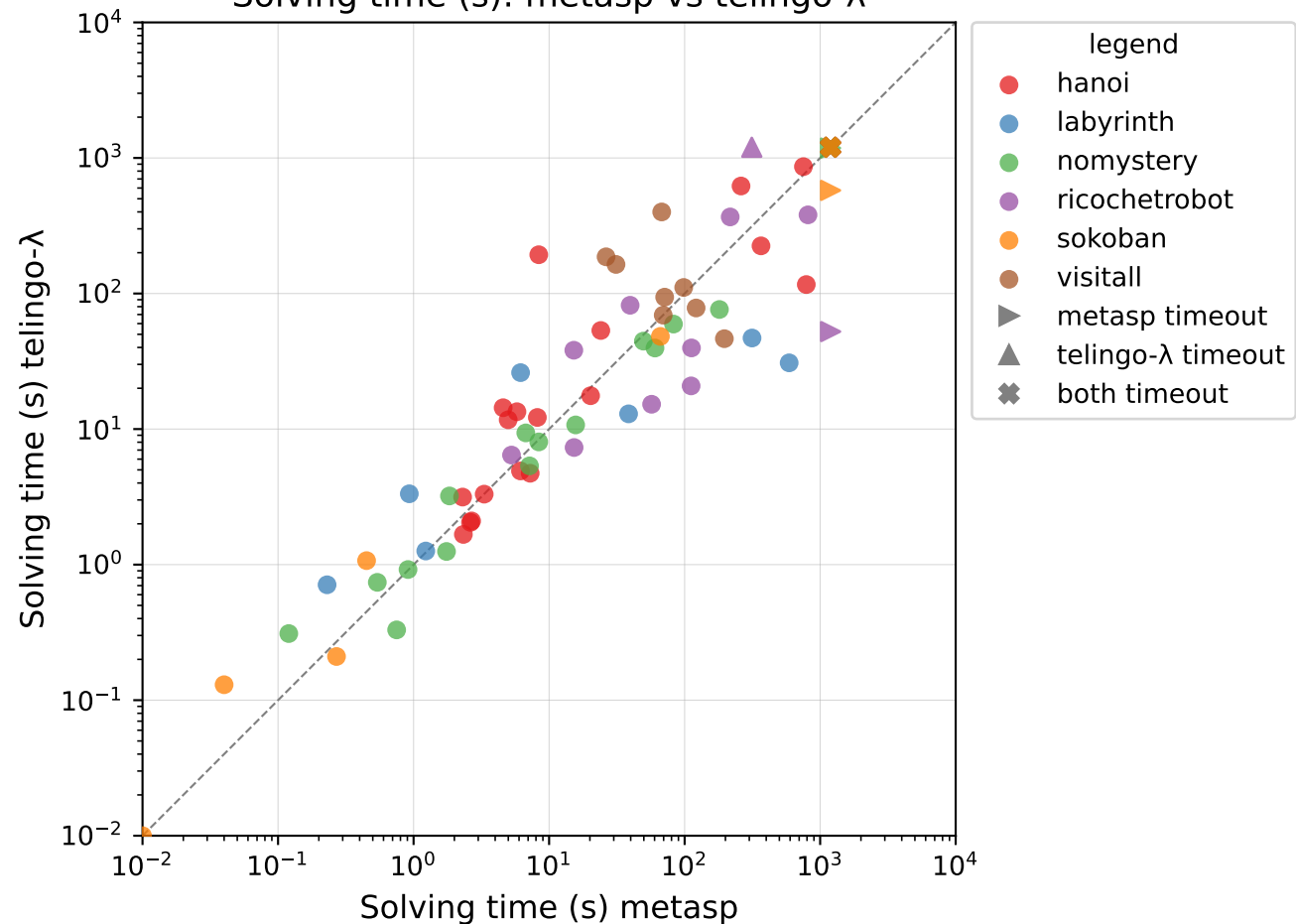
Solving time (s): metasp vs telingo- \lambda
