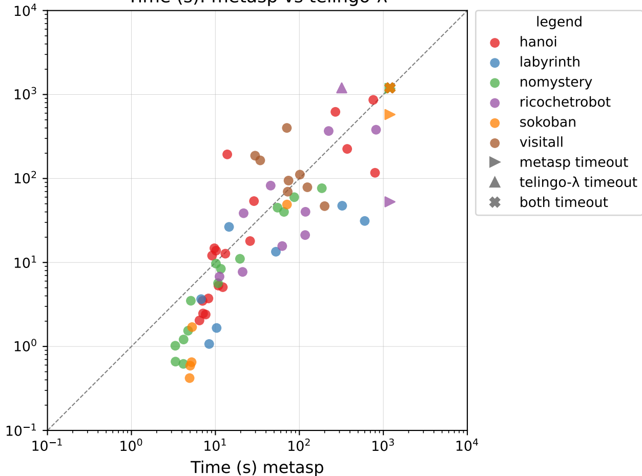
Time (s): metasp vs telingo- \lambda
