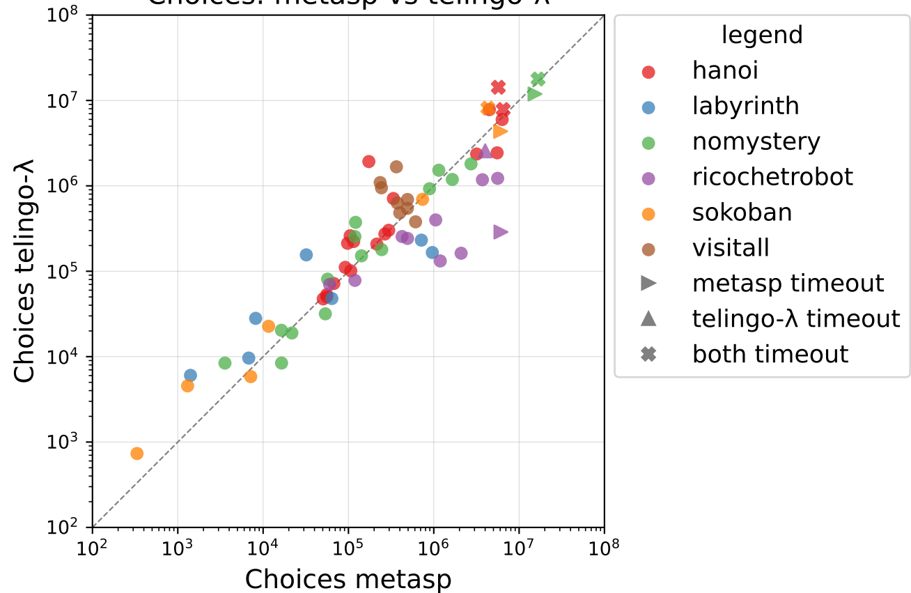
Choices: metasp vs telingo- \lambda
