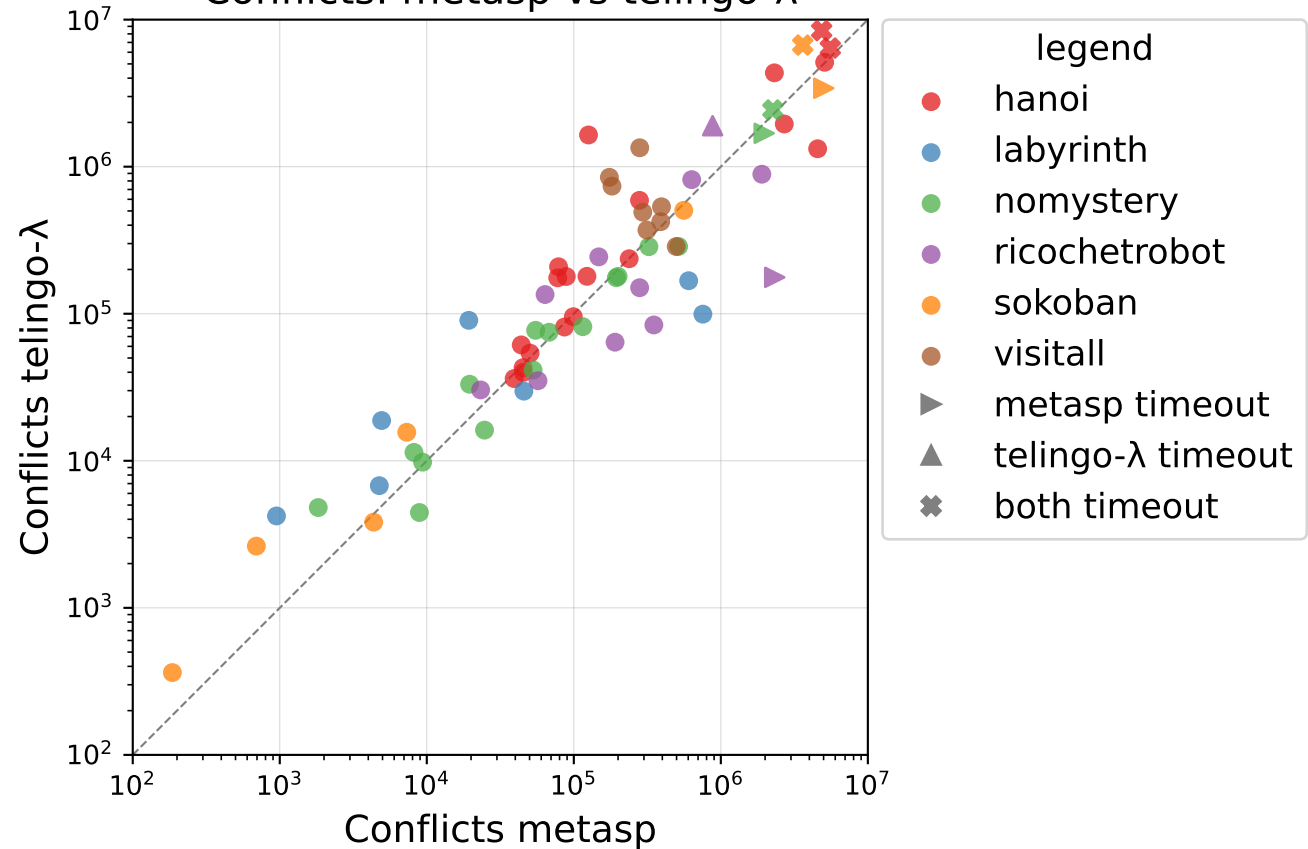
Conflicts: metasp vs tilingo-λ
