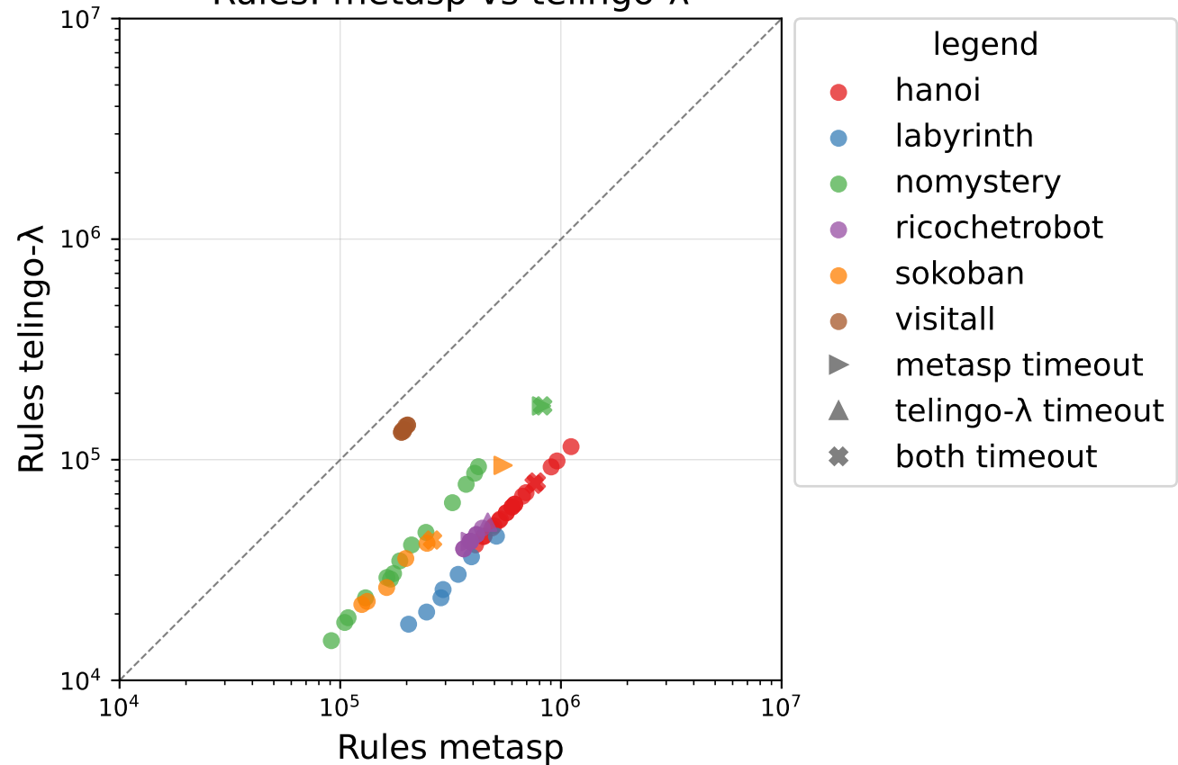
Rules: metasp vs telingo-λ
