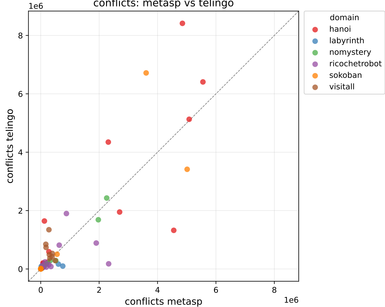
conflicts: metasp vs telingo
