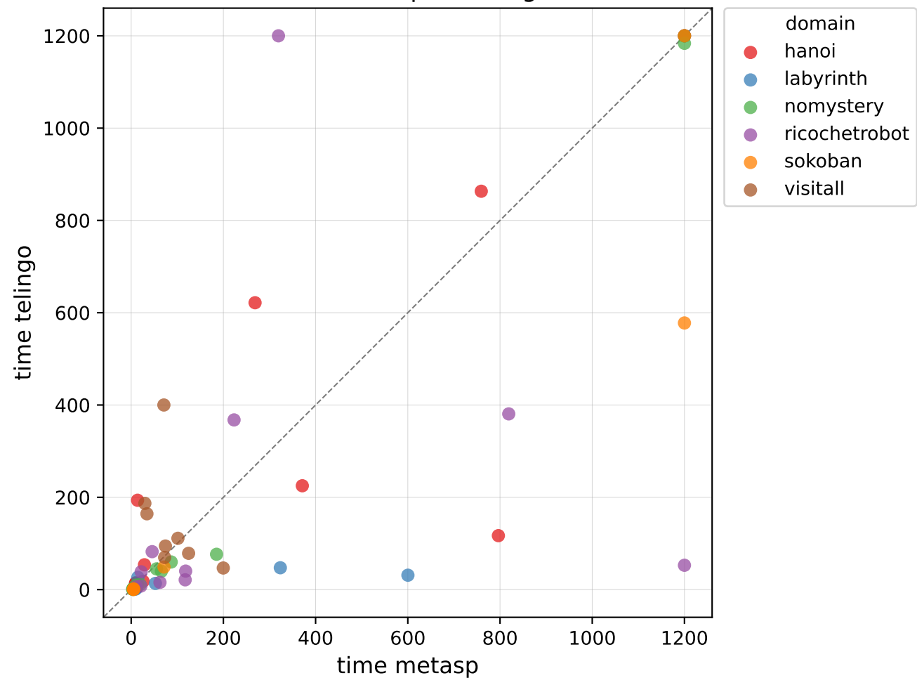
time: metasp vs telingo
