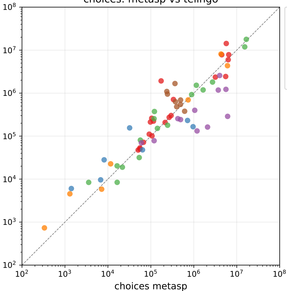
choices: metasp vs telingo
