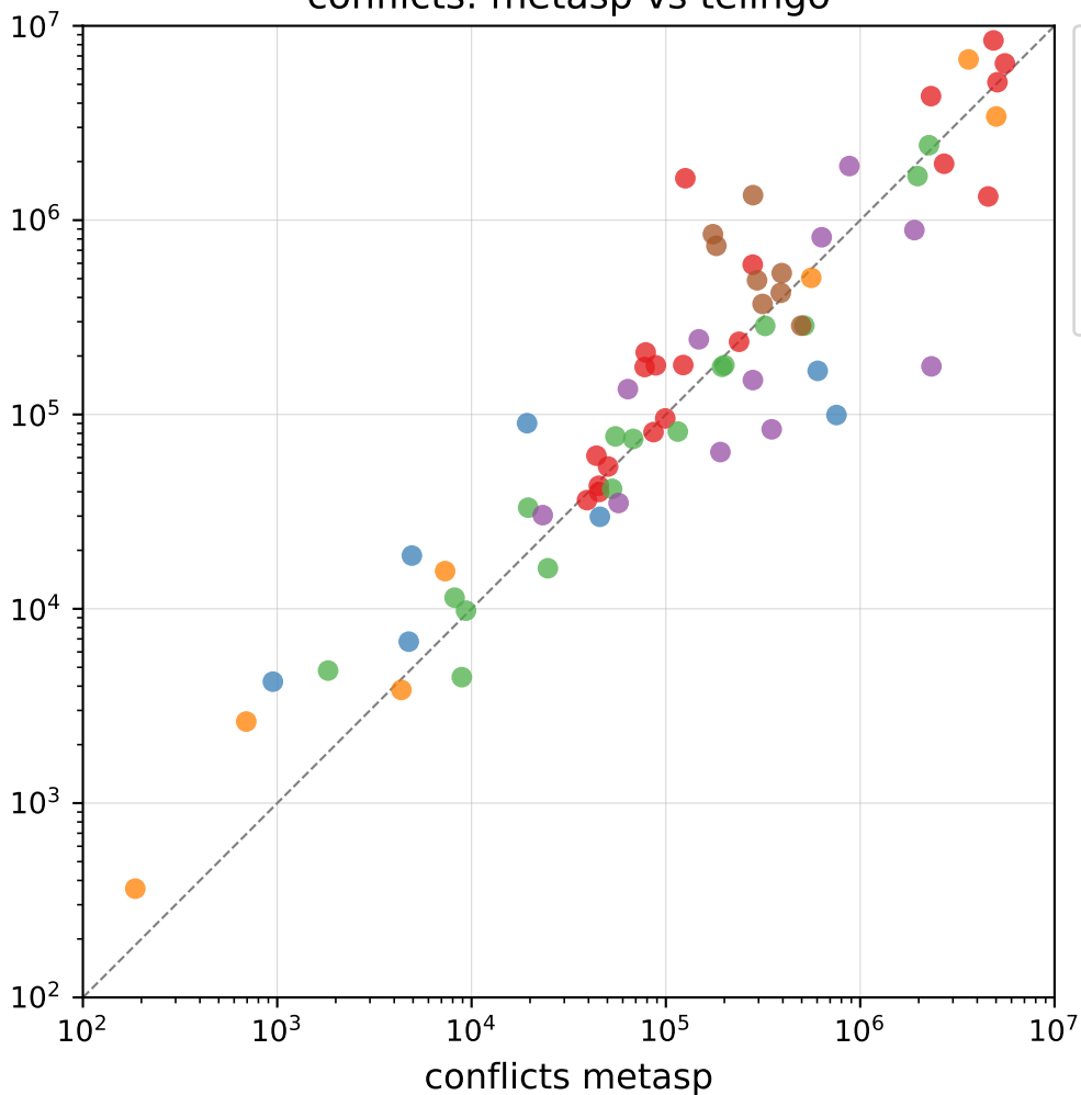
conflicts: metasp vs telingo
