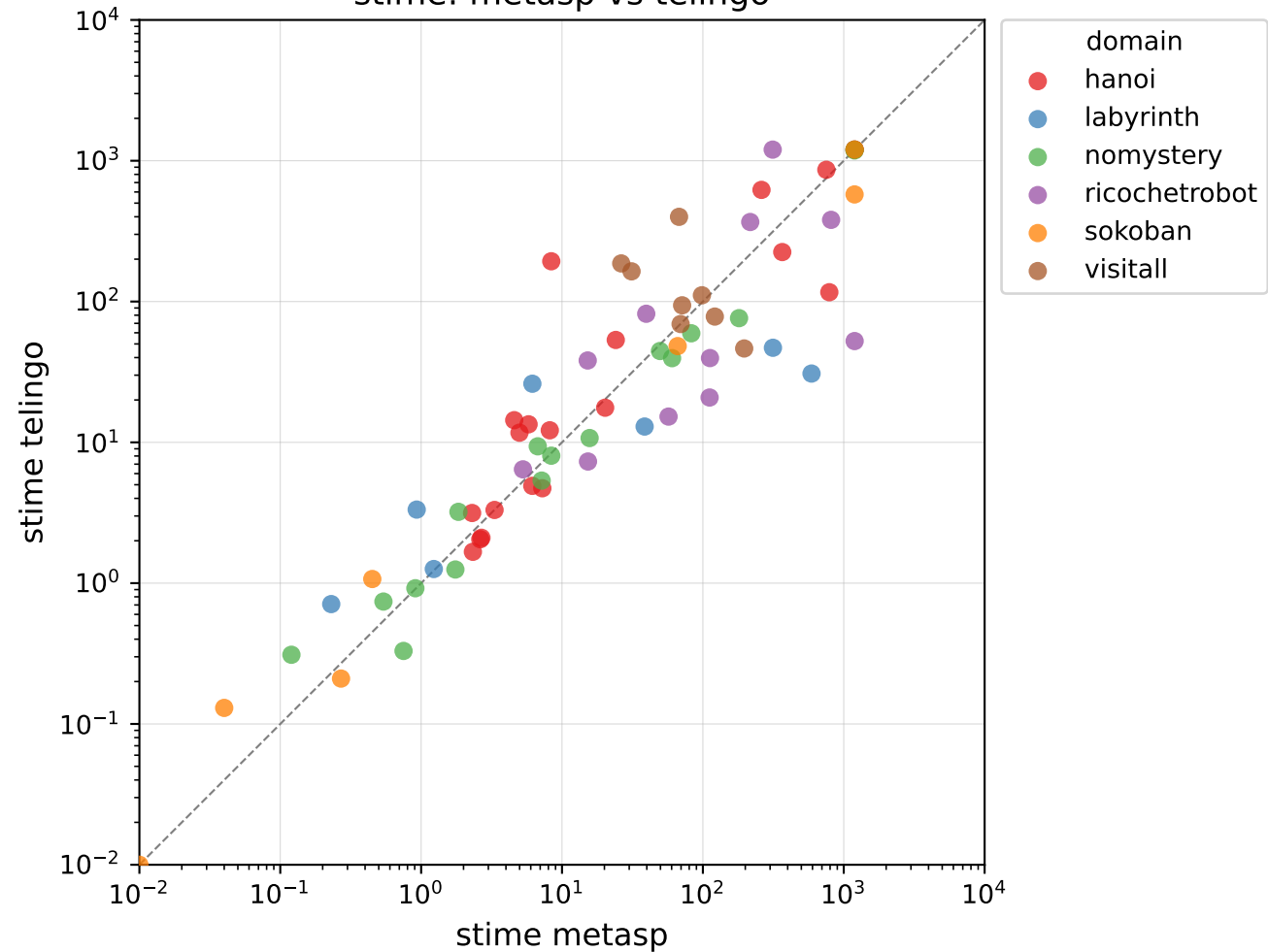
stime: metasp vs telingo
