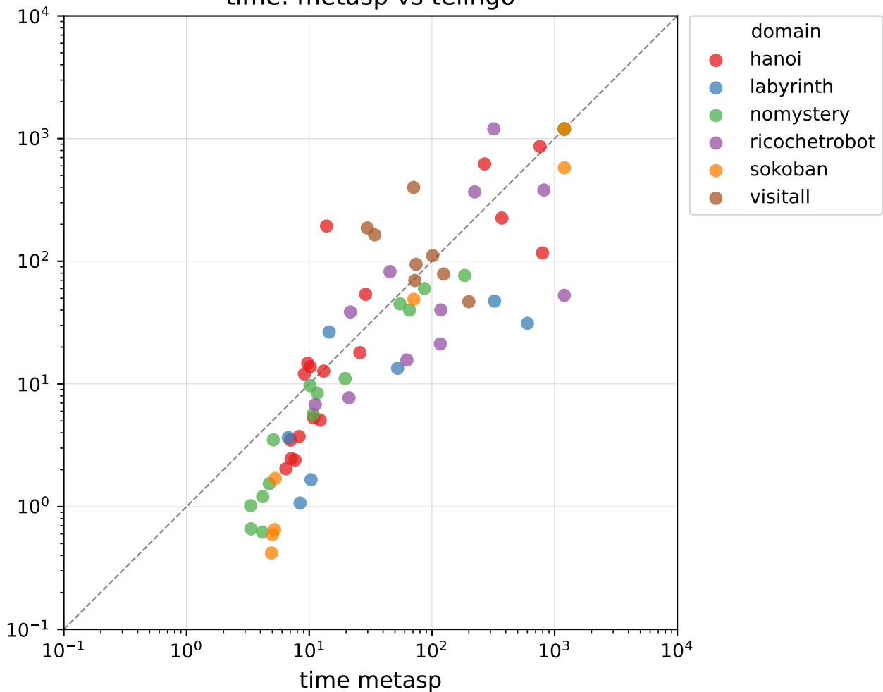
time: metasp vs telingo
