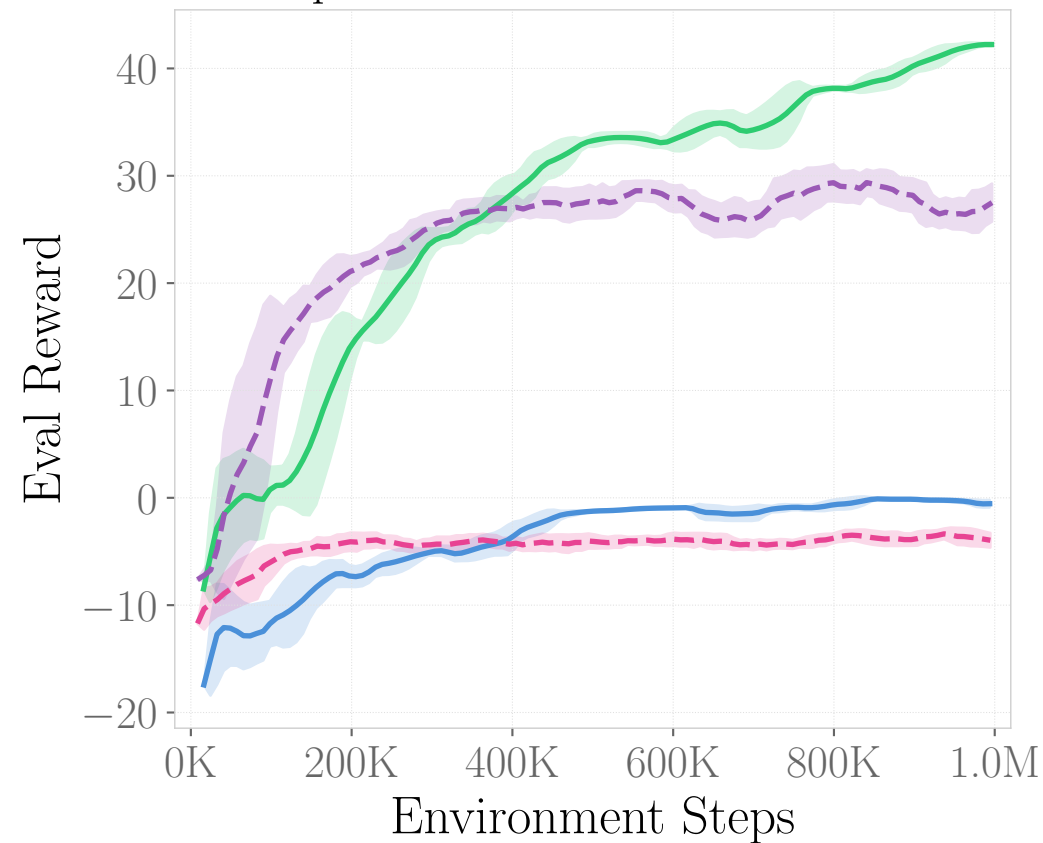
AlphaTransit vs End-to-End RL
