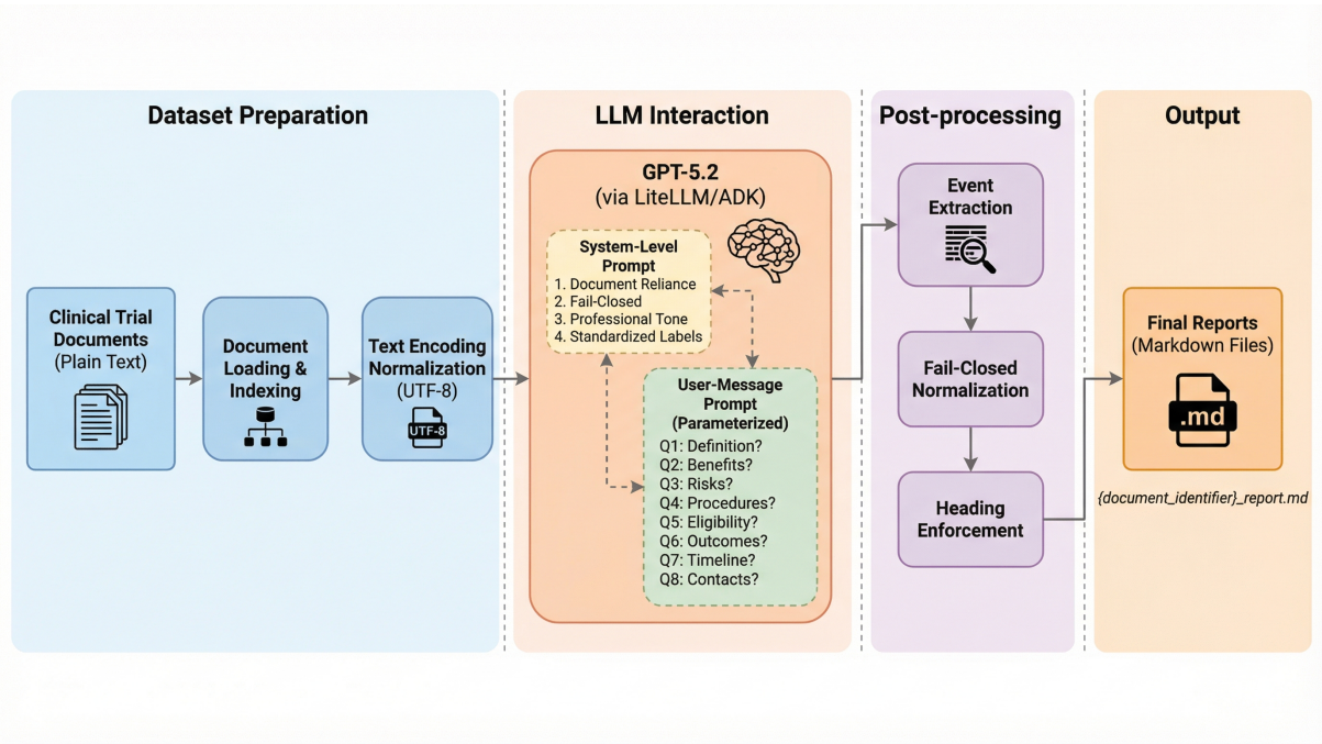
Figure 1: Overview of the AI-assisted summary generation pipeline. Clinical trial guidance documents are loaded and encoded (left), processed through GPT-5.2 via a two-tier prompting architecture (center), passed through three automated quality-control steps (right), and saved as structured Markdown reports (far right).
