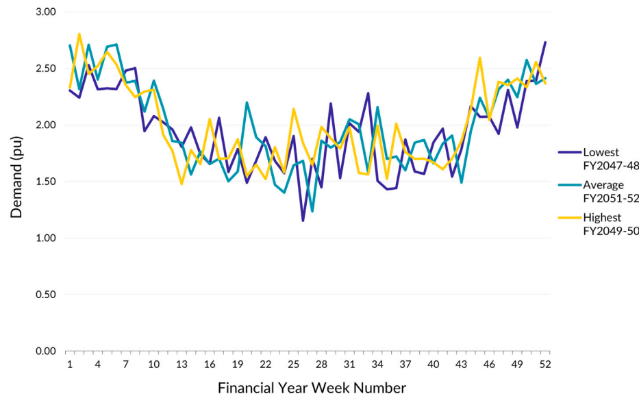
Fig. 7. Comparison of the weekly average demand across the best, worst and representative years within the forecast period. Demand is in per unit of the FY2024-25 average operational demand in SA (1300 MW).
