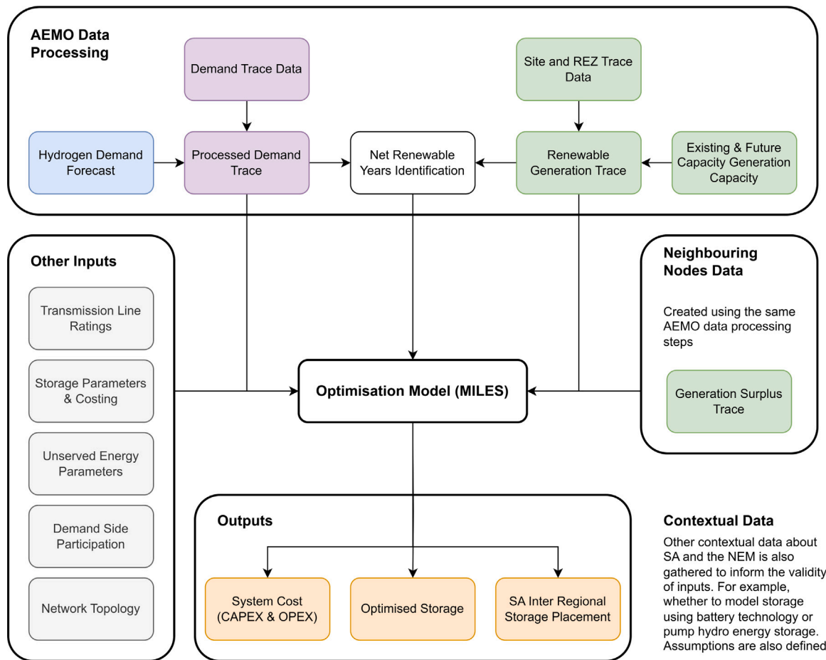
Fig. 2. Data processing workflow and model inputs.
