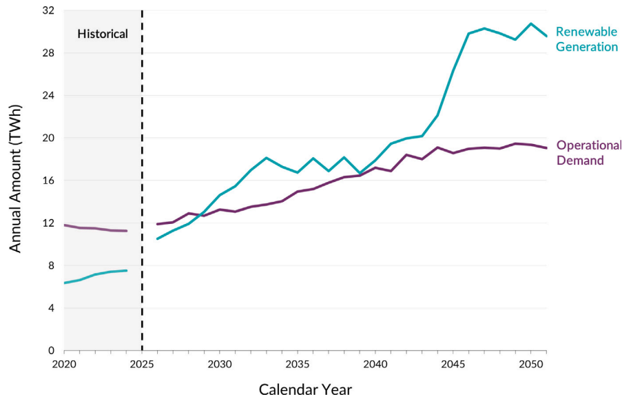
Fig. 4. Historical and forecast annual operational demand and renewable generation based on AEMO's 2024 ISP and latest hydrogen forecasts. Note that the current calendar year is not included as the data has not yet been released by AEMO.
