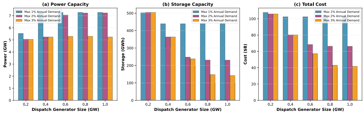
Fig. 10. Summary of the worst-case storage requirements for different generator dispatch sizes and percentages of demand met.
