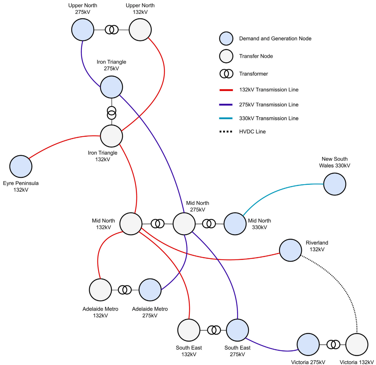
Fig. C.2. Nodal representation of the South Australian electricity grid.
