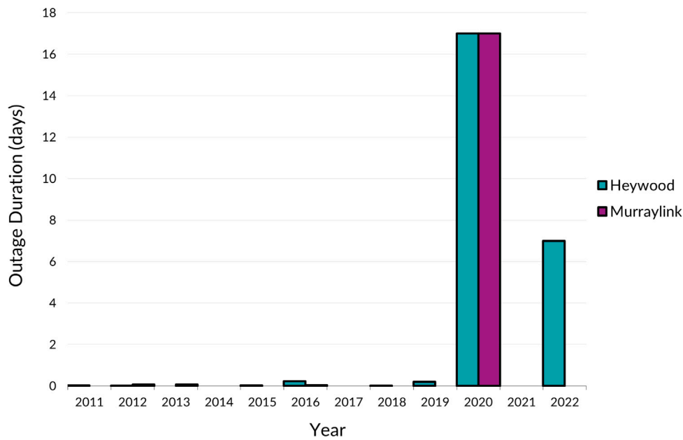
Fig. 1. Annual interconnector outage duration in South Australia.
