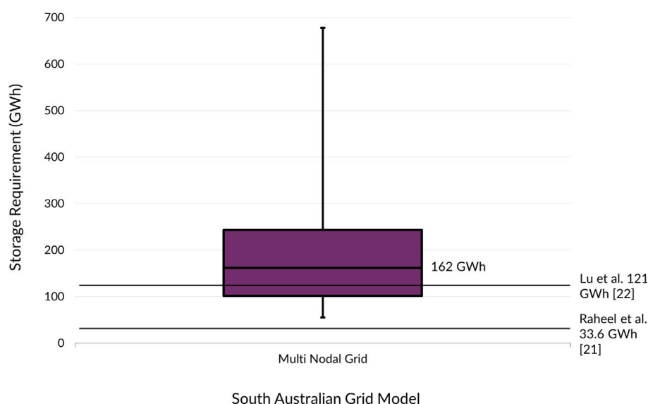
Fig. 12. Box and whisker plot comparing the storage requirement of all cases and years considered in the analysis. Previous research results are also displayed for comparison.
