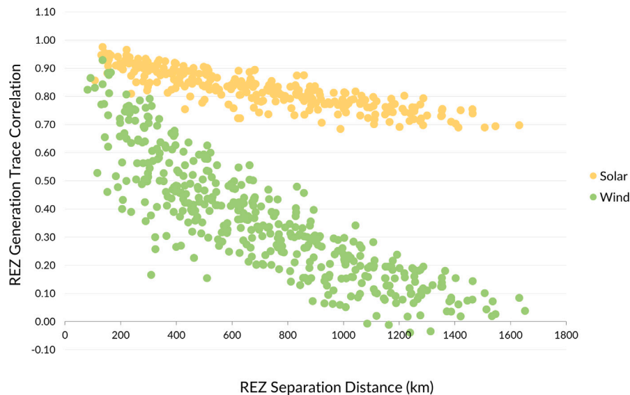
Fig. 9. Relationship between the generation trace correlation and distance of solar and wind REZs in SA, NSW, and Victoria.
