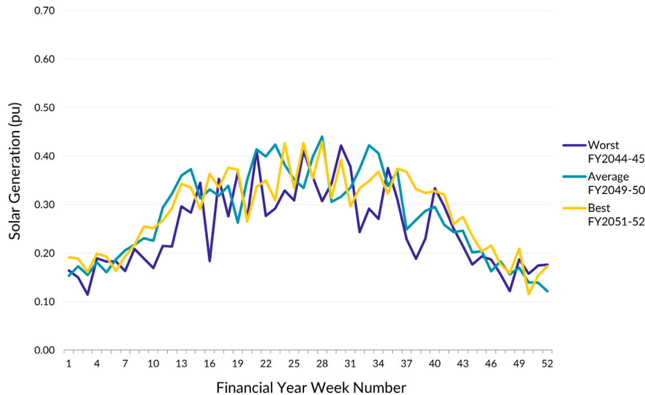
Fig. 5. Comparison of the weekly average solar generation across the best, worst and representative years within the forecast period.
