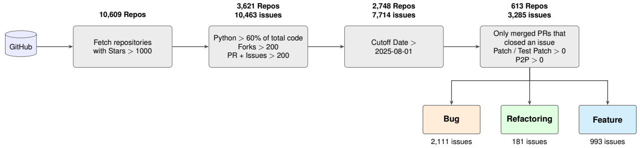
Fig. 2: Data collection pipeline. Starting from 10,609 GitHub repositories with more than 1,000 stars, we apply successive filters for language composition, repository activity, issue recency, and merge-based linking to produce 3,285 benchmark-ready instances across 613 repositories.
