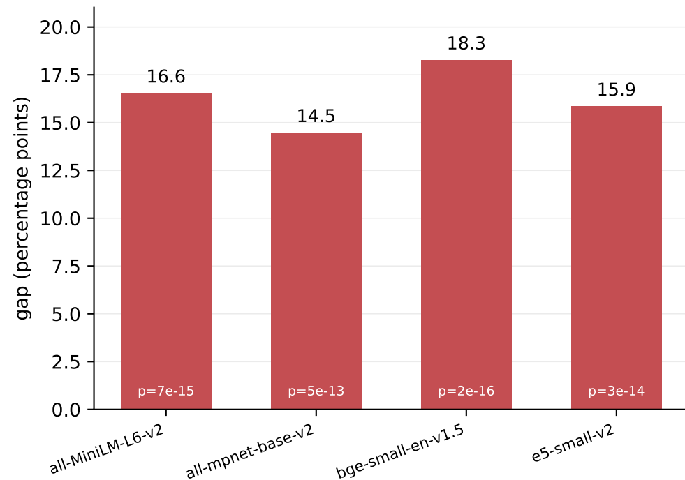
QASPER — granularity (B→C) (n=290)
