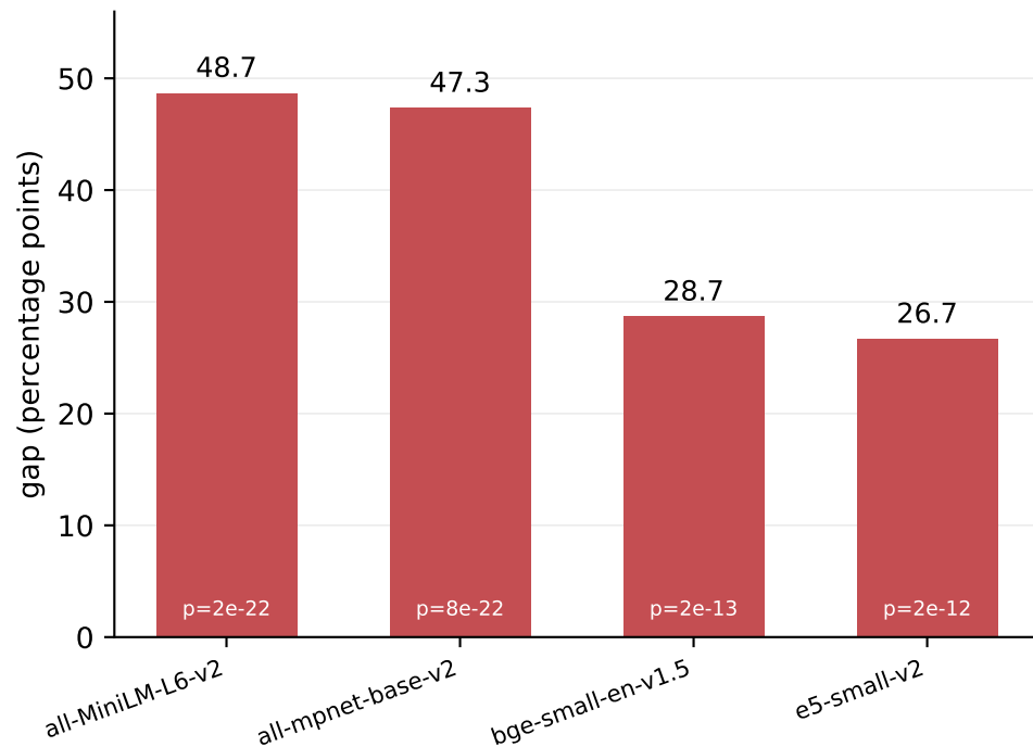
HotpotQA — quantifier (A→B) (n=150)
